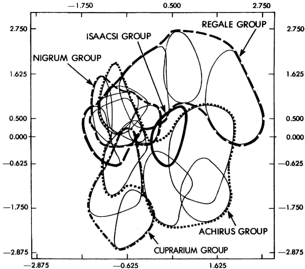
FIGURE 3.—Artist's rendering of plot of first two discriminant scores of selected proportional measurements for all species of Nannobranchium (see "Methods" for explanation). The species clusters are denoted by the solid thin lines. Envelopes for all species groups are denoted by separately labeled bold solid and dashed curves.
