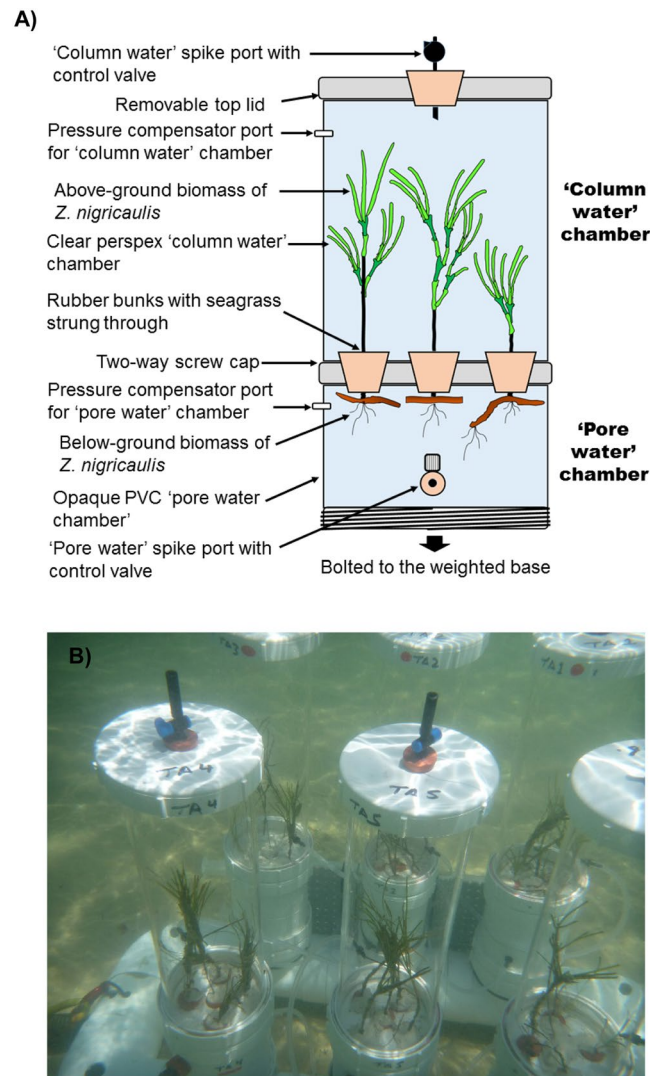
Figure 3. Benthic chambers used for translocation studies. (A) Schematic cross-sectional diagram of the translocation chamber with its individual components, and (B) Close up of the top chamber with the two-way screw cap. Individual plants are threaded through a rubber bung in such a way that the above-ground biomass remain in the top clear Perspex chamber (column water) and the below-ground biomass remains in the chamber below (pore water).
