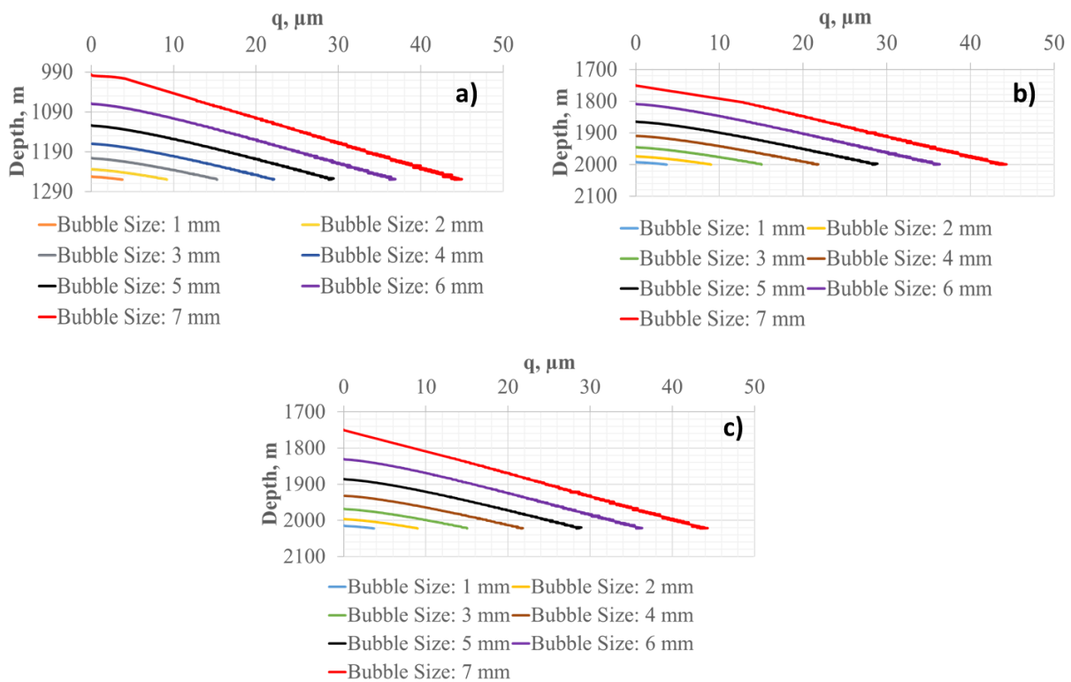
Figure 2. Rate of the gas exchange ( q ) at different bubble sizes for a) Thessaloniki MV b) Kazan MV c) Amsterdam MV.
