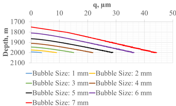
Figure 3. Rate of the gas exchange ( q ) at different bubble sizes for Napoli MV and Milano MV.
