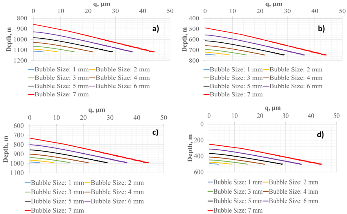
Figure 4. Rate of the gas exchange ( q ) at different bubble sizes for a) Amon MV b) Osiris MV c) Isis MV d) North Alex MV.
