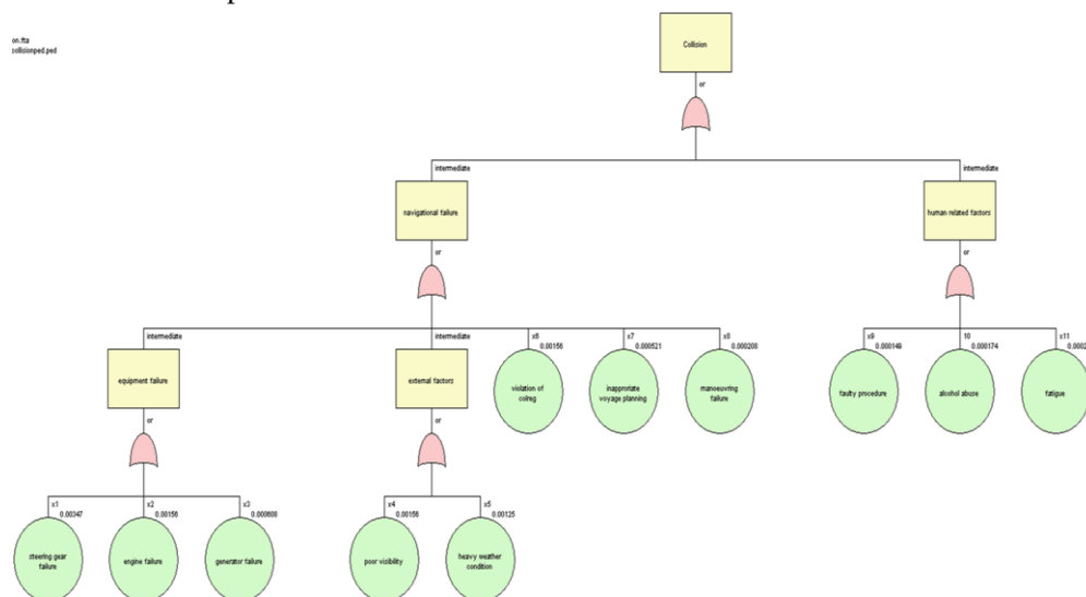
Figure 4. Fault tree for collision accidents
