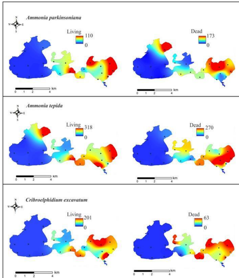
Figure 3. Species distribution of living and dead density (ind 50 mL -1 ) of A. parkinsoniana , A. tepida and C. excavatum in SLS.
