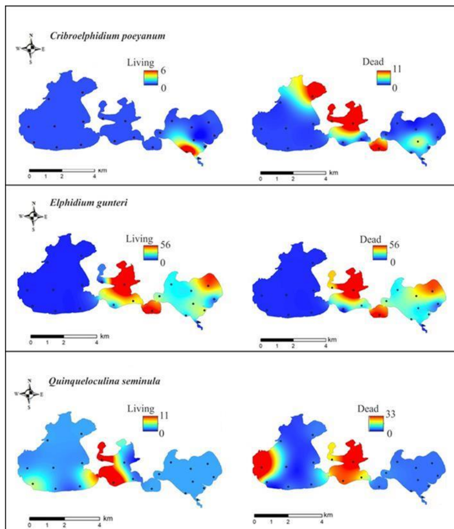
Figure 4. Species distribution of living and dead density (ind 50 mL -1 ) of C. poeyanum , E. gunteri and Q. seminula in SLS.
