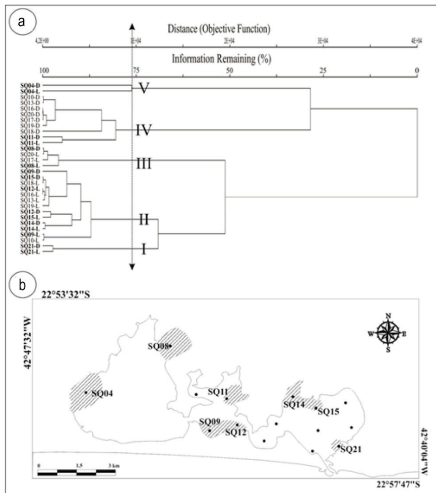
Figure 6. Q-mode Cluster Analysis of stations in the SLS based on relative abundance of living (L) and dead (D) foraminifera (Appendix 2). a) Five groups were defined considering 78% of similarity. In bold are the stations where the L- and D-assemblages compose the same group, b) the distribution map of the stations where the L and D-assemblages have at least 78% similarity according to the cluster analysis results.
