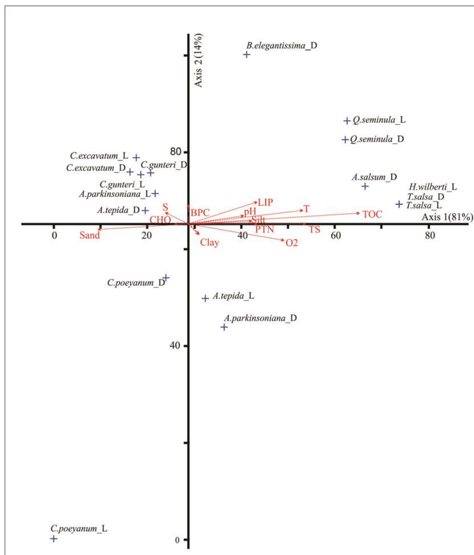
Figure 5. DCA analysis relating the living (L) and dead (D) Foraminifera species with the abiotic parameters in SLS. BPC: the total of biopolymers, CHO: carbohydrates, LIP: lipids, PTN: proteins, TS: total sulfur, TOC: total organic carbon, S: salinity, T: temperature.
