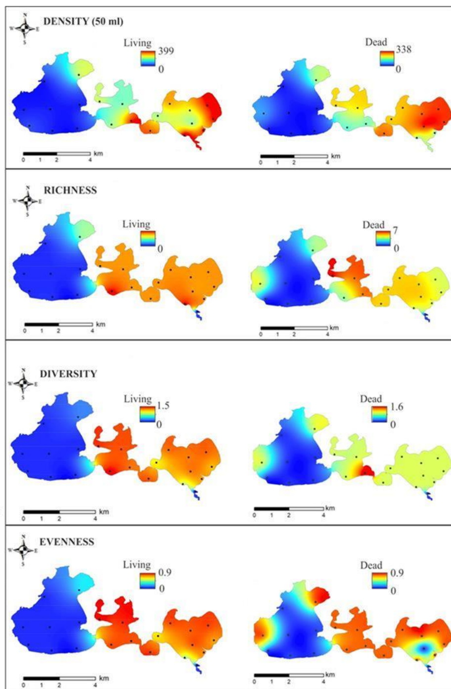
Figure 2. Distribution of living and dead foraminiferal density (ind 50 mL -1 ), species richness, diversity of Shannon and evenness in SLS.
