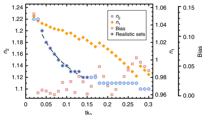
Fig. 3 Realistic sets of coated-sphere model parameters. Combinations of coat thickness ( tk_2 ) and refractive index ( n_2 ) that minimise the systematic error (Bias) of predictions for b_{bp} coefficients at 532 nm using a coated-sphere model with respect to in-situ optical measurements. tk_2 is expressed as a fraction of the radius of the modelled spherical particle. The volume-averaged refractive index n_1 is set equal to 1.06. Variations of the refractive index of the core ( n_2 ) as a function of tk_2 and n_2 are also shown. Black stars indicate the 12 realistic combinations of coated-model parameters selected for particle populations at the ocean surface (5 m) and at the DCM level. The dashed line is the fit to the realistic sets of coated-sphere parameters and corresponds to n_2 = 1.013 (\pm 0.003) tk_2^{-0.051 (\pm 0.002)} ( r = 0.99 , p < 0.01 , N = 12 )
