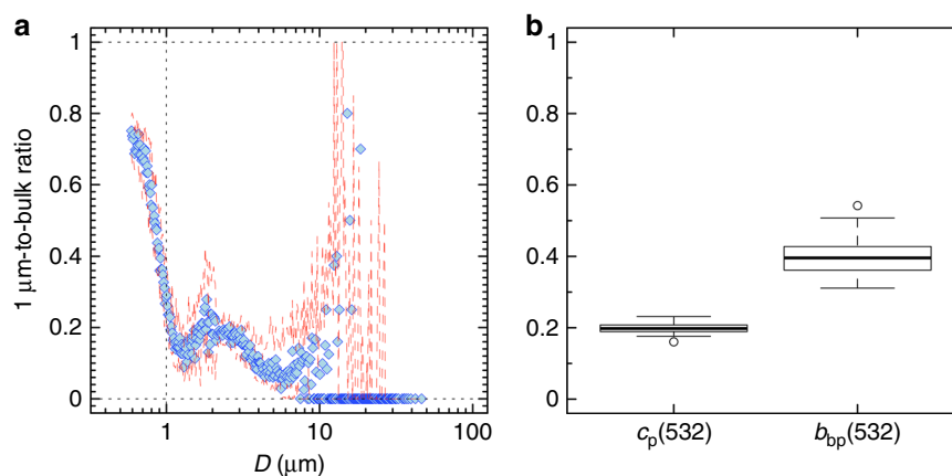
Fig. 6 The optical contribution of submicron particles after 1 \mu\text{m} filtration. a Ratio of particle size distributions measured after and before filtration of 5-m water samples through a 1- \mu\text{m} filter as a function of the particle diameter ( D , units of \mu\text{m} ). Each point is the median of all ratios for samples collected during the AMT26 cruise ( N = 22 ; Supplementary Fig. 1) for a given particle diameter. Red dashed lines represent the first and third quartiles. b Boxplot for the corresponding 1 \mu\text{m} -to-bulk ratios of c_p and b_{bp} coefficients at 532 nm. The thick black line indicates the median value. Upper and lower side of each box are the third and first quartiles, respectively. Vertical bars represent minimum and maximum values. Open circles are outliers
