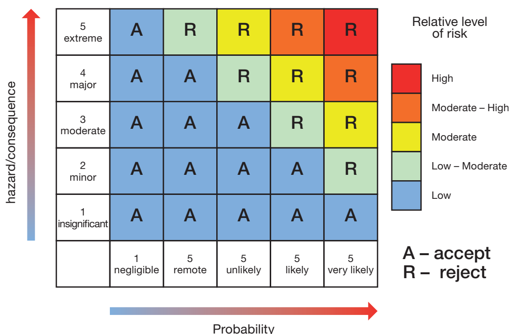
Figure 8.3 Risk matrix indicating the acceptable level of risk for a hypothetical hazard, illustrated in Figure 8.2 (based on GESAMP 2008)
