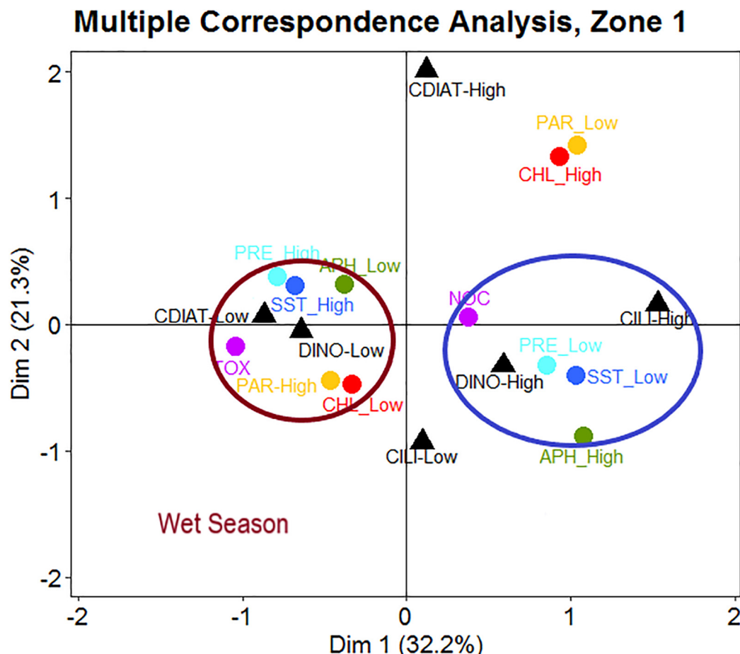
FIGURE 7 | In Zone 1, occurrences of toxic HABs (TOX) linked to low concentrations of dinoflagellates (DINO) and centric diatoms (CDIAT) are associated with high levels of sea surface temperature (SST), precipitation (PRE), and photosynthetic active radiation (PAR) as well as low levels of absorption coefficient of phytoplankton at 443 nm (aph) and chlorophyll a (chl- a ) appearing during the wet season. Events of non-toxic HABs (NOC) appearing with high concentrations of DINO and ciliates (CILI) are associated with low levels of SST and PRE, accompanied by high values of aph.
