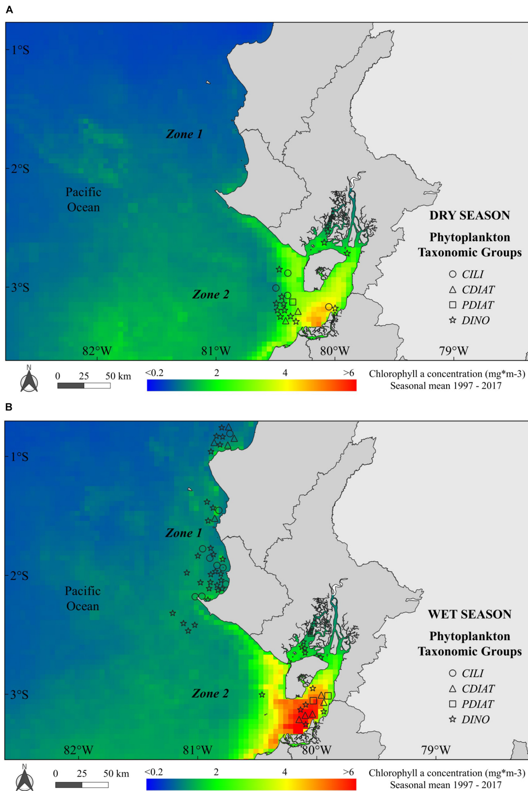
FIGURE 3 | Spatial distribution of occurrences of phytoplankton taxonomic groups (PTGs: ciliates, centric diatoms, pennate diatoms and dinoflagellates) along the Ecuadorian coast during (A) the dry season—occurrences of PTGs and (B) the wet season—occurrences of PTGs in Zones 1 and 2 of the study area. Background colors show the seasonal mean of chlorophyll a for the dry and wet seasons.
