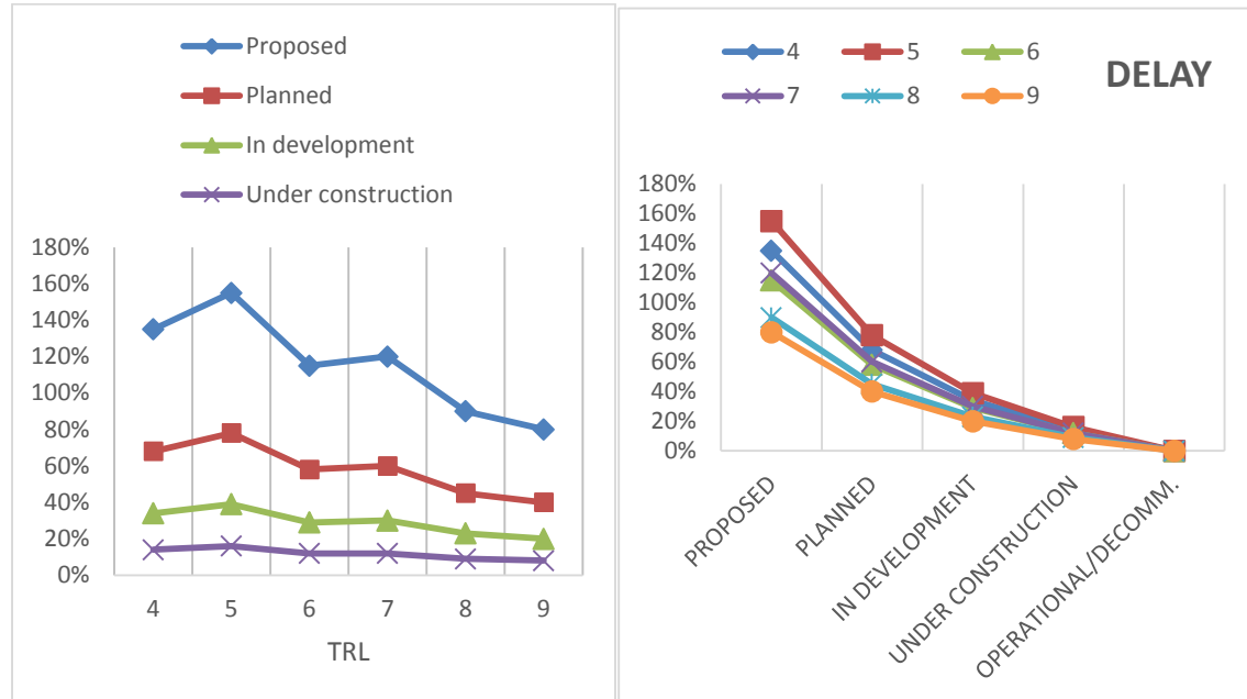
Figure 6 - Delay rate based on TRL and Status, to be used in the medium and pessimistic scenario (not modified by technology)
