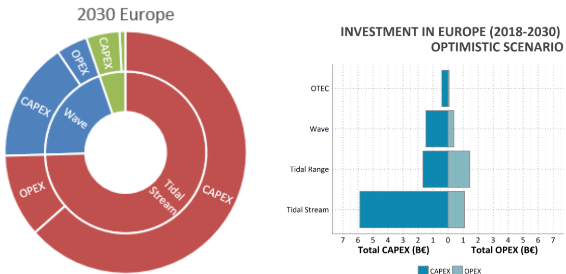
Figure 37 - Breakdown of investments by technology and cost type
