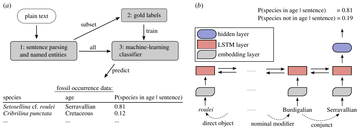
Figure 1. (a) The general workflow for automatic information extraction of fossil occurrence data. (b) The machine-learning classifier. A bidirectional long short-term memory (LSTM) recurrent neural network, with the first example candidate as input. The numbers given are illustrative. Dashed arrows indicate dependency grammar links. See electronic supplementary material for details on the classifier. The figure style is inspired by Miwa & Bansal [23]. (Online version in colour.)
