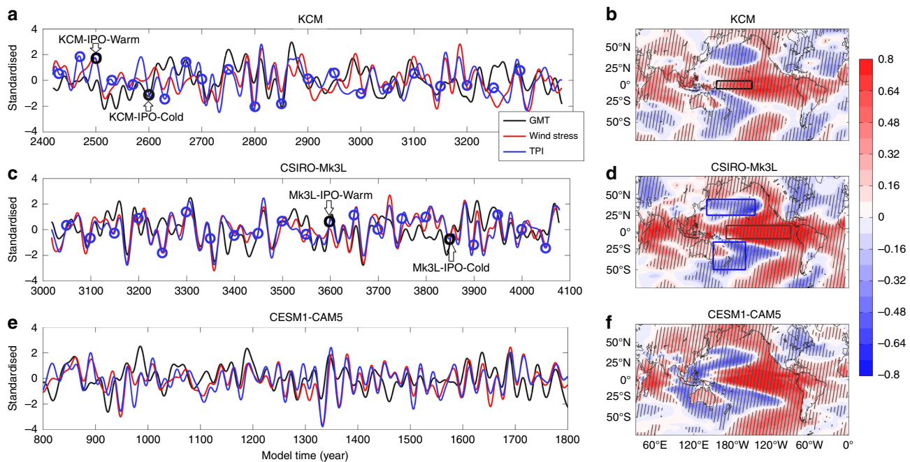
Fig. 1 Time series of tropical Pacific zonal wind stress, globally averaged SAT, and the Tripole Index in the three climate models. Time series of low-frequency fluctuations (11-yr low passed filter) in (a, c, e) zonal wind stress over western equatorial Pacific (red solid lines), globally averaged SAT (black solid lines), and the Tripole Index (TPI; blue solid lines) from a KCM, c Mk3L, and e CESM-CAM5 control runs (all time series have been standardized). Blue (black) circles in a and c denote the initial year of the KCM-ICs (the KCM-IPO-Cold and the KCM-IPO-Warm) and the Mk3L-ICs (the Mk3L-IPO-Cold and the Mk3L-IPO-Warm) global warming simulations, respectively. b, d, f panels display the corresponding correlation between low-frequency fluctuations in the equatorial zonal wind stress (11-yr low passed filter) and local SAT anomalies computed from the control runs. Boxes on d indicate locations used for the calculation of the TPI. Hatching in b, d, f show where the correlation is statistically significant at 99% confidence level (accounting for autocorrelation in the time series)
