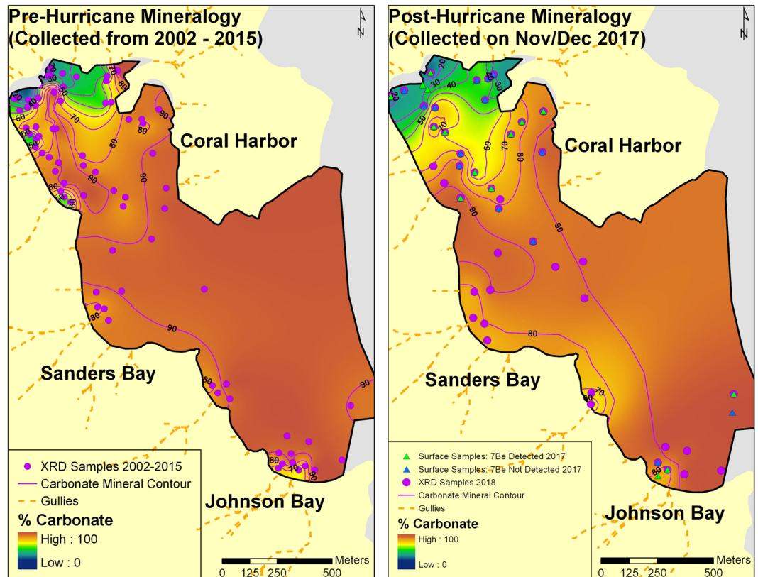
Figure 4. Surficial mineralogy of Coral Bay, St. John pre (left) and post (right) September 2017 Hurricanes Irma, Jose, and Maria. The post hurricane map also includes samples run for ^7\text{Be} (triangles). Both pre- and post-storms, the seafloor was predominantly carbonate while there was some intrusion of terrestrial material following the hurricanes in northern Coral Harbor (right). Mineralogy was determined by XRD (X-Ray Diffraction).
