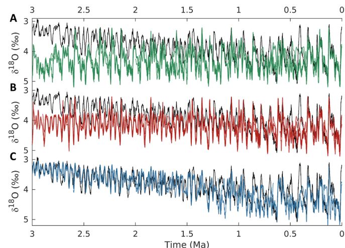
Fig. 6. External drivers and model response. Modeled benthic \delta^{18}\text{O} compared to observations (black) (3) for (A) simulations driven only by variations in orbital configuration, (B) simulations driven by orbital forcing and optimal regolith removal scenario (red), and (C) simulations driven by orbital forcing and optimal volcanic outgassing scenario (blue).
