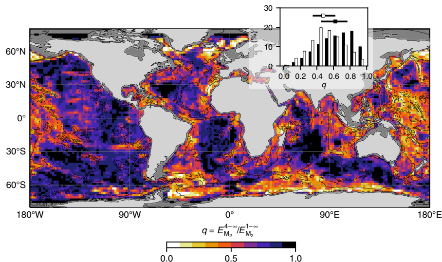
Fig. 5 Geography of the ratio q of local energy dissipation to total energy conversion. The ratio q is here defined as q = E_{M_2}^{4-\infty} / E_{M_2}^{1-\infty} , and is binned in 2^\circ \times 2^\circ squares for visual purposes. Inset bar-plot represents histograms of (black) seafloor area and (white) E_{M_2}^{1-\infty} binned as a function of q , and error bars represent the 25th and 75th percentiles on both sides of the median (square)
