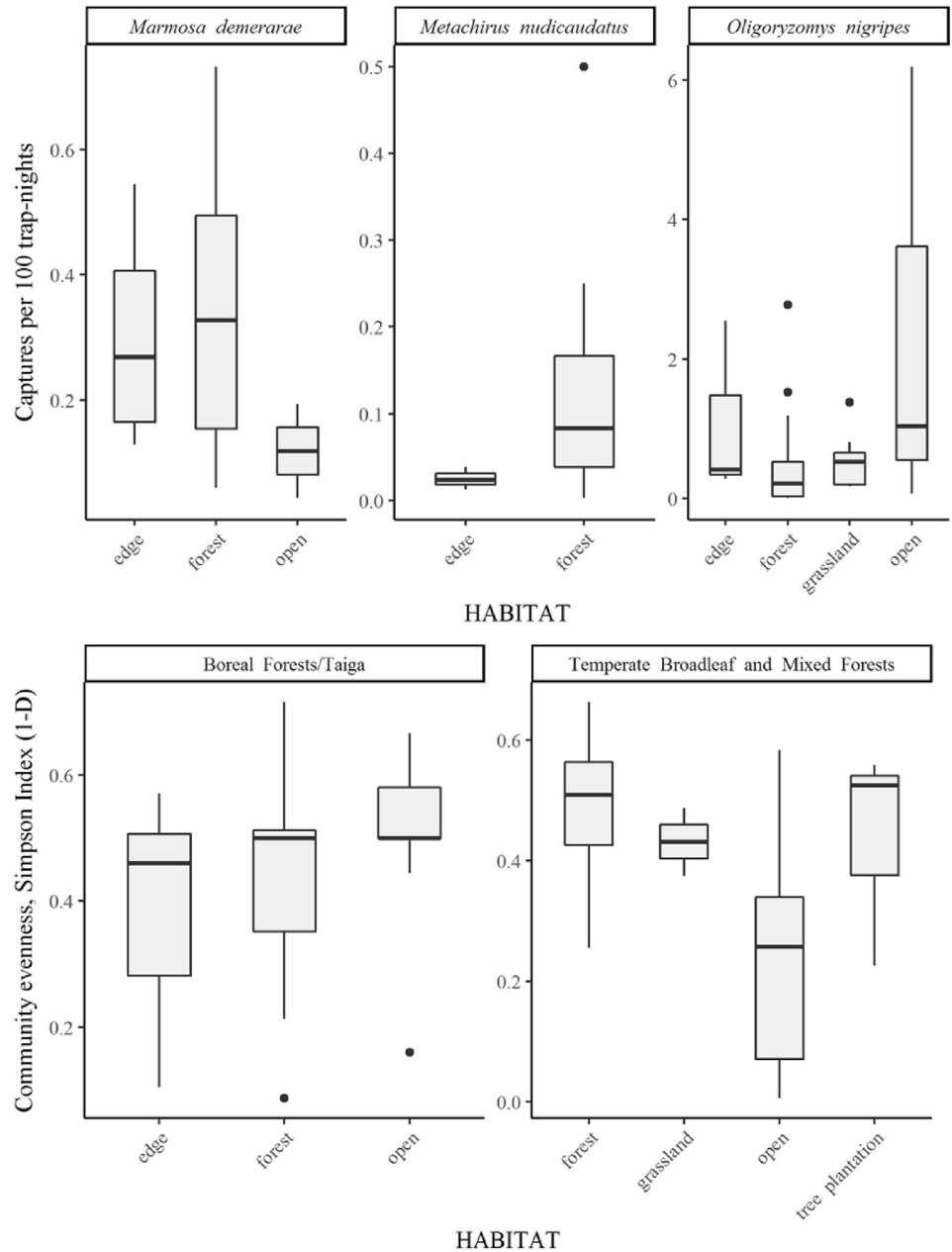
Fig. 2. Per-habitat differences in the captures per 100 trap-nights of three Neotropical small mammal species (superior) and in the evenness of non-volant small mammal communities in two Nearctic biomes (inferior).
