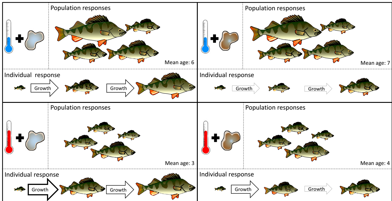
FIGURE 6 Fish biomass production in warmer and darker lakes. As the water gets warmer and browner, fish biomass production decreases through different pathways. With warming alone (from top to bottom left), population biomass decreases, and there is a shift toward smaller and younger individuals. Young but not old individuals exhibit higher growth rates. As lakes get browner (but not warmer; from top left to top right), mean age increases slightly, but there is no shift in population biomass or mean length. Body growth of both small and large individuals is reduced. As lakes get both warmer and browner (from top left to bottom right), there is a strong decrease in fish biomass production due to reduced population biomass, a shift toward smaller and younger individuals and slower body growth
