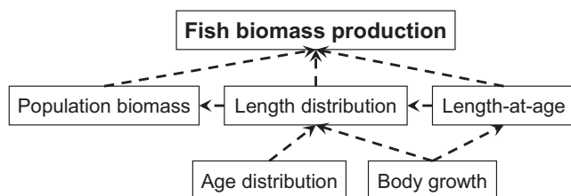
FIGURE 1 Fish biomass production and its underlying individual- and population-level attributes. Individual body growth underlies changes in length-at-age, and together with population age-distribution (mean age, skewness in age), also changes in population length distributions (mean length, skewness in length), fish biomass, and ultimately fish biomass production. The net effect of warming and browning on fish biomass production may thus depend on changes in interlinked variables responding to warming and browning both at the level of individuals and of populations
