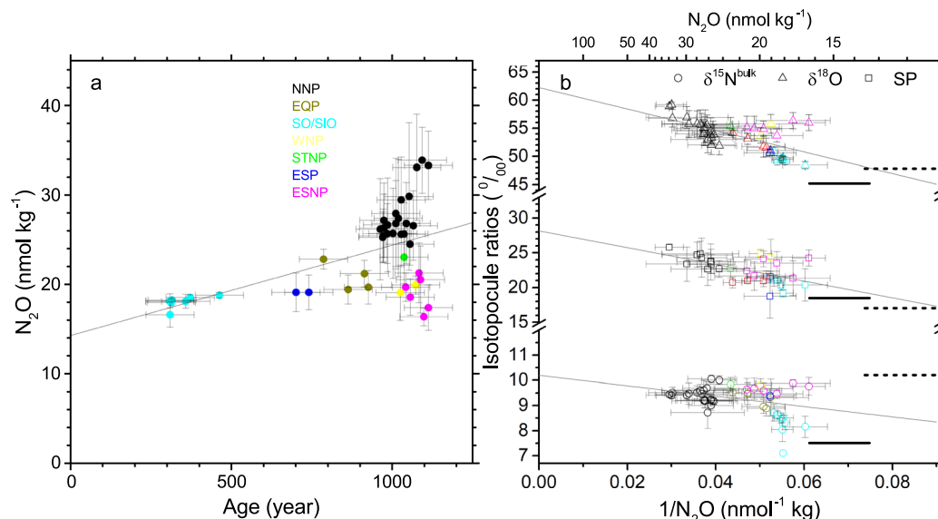
Figure 5. Concentration and isotopocule ratios of \text{N}_2\text{O} for deep water (depth >2000 m) in nine oceanic regions and their relation with circulation age of seawater. (a,b) Relation between circulation age and \text{N}_2\text{O} concentration (a) and relation between inverse concentration and isotopocule ratios of \text{N}_2\text{O} (b) . Each symbol denotes the average for the deep water at each station. Error bars for concentration and isotopocule ratios show one standard deviation while those for age are reported estimated error 26 . Solid and broken horizontal lines in panel b respectively show the values expected when the surface water in the subduction region is equilibrated with modern and preindustrial atmosphere 31 . Correlation coefficients of regression lines and probabilities of null hypothesis in ANOVA are as follows. In panel a, r = 0.55 , p = 1.3 \times 10^{-4} ; in panel b, \delta^{15}\text{N}^{\text{bulk}} , r = -0.38 , p = 1.3 \times 10^{-2} ; \delta^{18}\text{O} , r = -0.65 , p = 2.3 \times 10^{-6} ; SP, r = -0.56 , p = 1.4 \times 10^{-3} .
