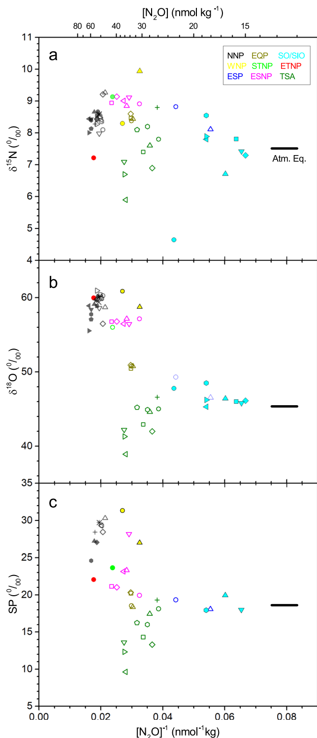
Figure 3. Comparison of isotopocule ratios of \text{N}_2\text{O} at concentration maximum in nine oceanic regions. (a–c) Relations between inverse concentration and \delta^{15}\text{N}^{\text{bulk}} (a), \delta^{18}\text{O} (b), and \text{SP} (c). Colors and types of symbols are as shown in Fig. 2. Horizontal solid lines show values of dissolved \text{N}_2\text{O} when the seawater is equilibrated with the atmosphere.
