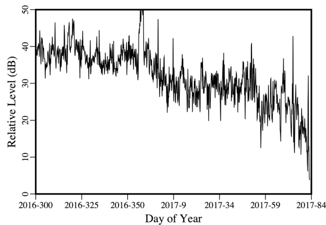
Figure 8. Peak intensity of the received signal from the distant source, which decreases as scattering features develop on the underside of the ice.
