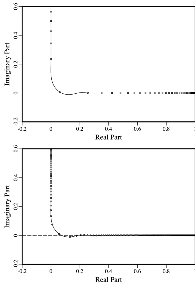
Figure 3. Mappings of the eigenvalues (which are shown as small circles) by rotated rational approximations. At 50 Hz (top) all of the eigenvalues are mapped on or above the real axis. At 250 Hz, a few of the eigenvalues are mapped below the real axis.
