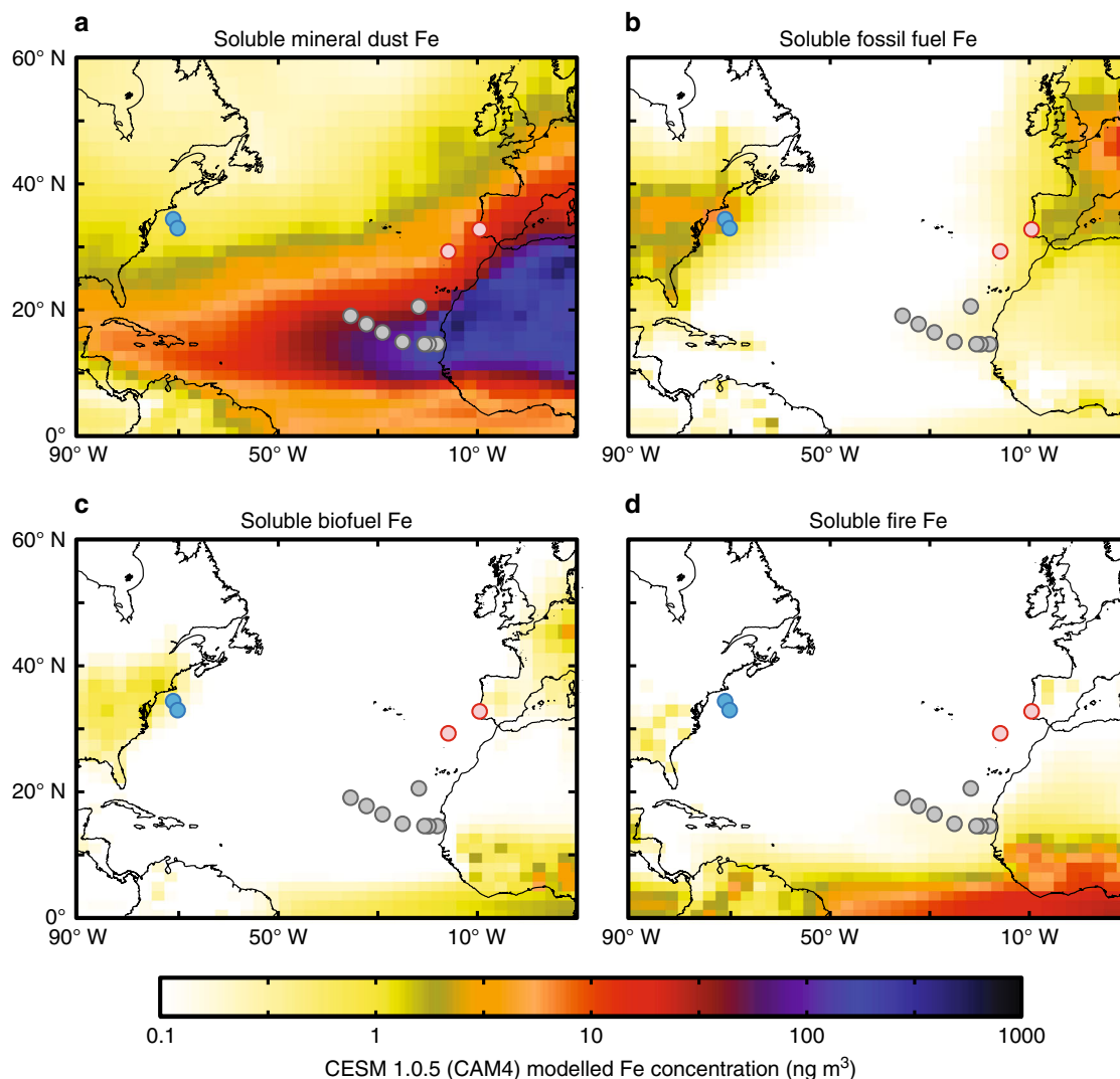
Fig. 4 Modeled aerosol Fe for the North Atlantic. CAM4 baseline model soluble aerosol Fe (combined October + November deposition) of aerosol Fe concentration for crustal mineral dust, fossil fuel, biofuels, and fire, with sampling locations in this study shown. Panels show soluble aerosol Fe concentration output for a mineral dust, b fossil fuel, c biofuel, and d fire from the Community Earth System Model (CESM 1.0.5) with the Community Atmosphere Model (CAM4) bulk aerosol model, using intermediate complexity soluble atmospheric processing (baseline CAM4 scenario) 49,50 . GA03 sampling locations are color coded as in Fig. 1
