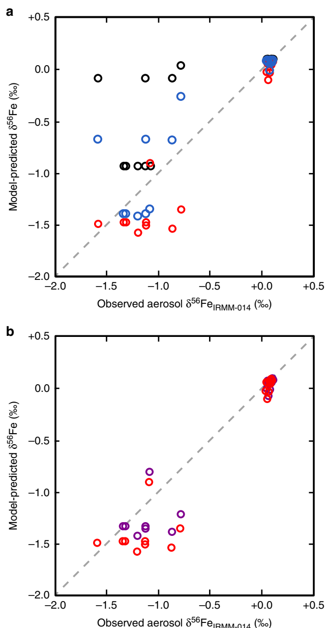
Fig. 5 Comparison of GA03 observations with model predictions. Black circles denote output from CAM4 baseline model scenario of Scanza et al. 49 with monthly average output and end members of +0.09\text{‰} for dust and -1.6\text{‰} for anthropogenic Fe, and shows poor agreement. In a , agreement is improved by changing model to use daily mineral dust to capture dust storms and reduced dust source solubilization (from 25 to 10%) (blue circles). Agreement is further improved in a by using 5\times anthropogenic emissions, to generate an isotope-refined model scenario (CAM4 isotope-refined scenario) which best matches GA03 observations (red circles). The anthropogenic endmember was also optimized in b to provide best fit between model and observations (see main text; red points are with an anthropogenic \delta^{56}\text{Fe} endmember of -1.6 , purple circles are with an optimized anthropogenic \delta^{56}\text{Fe} endmember of -1.4\text{‰} )
