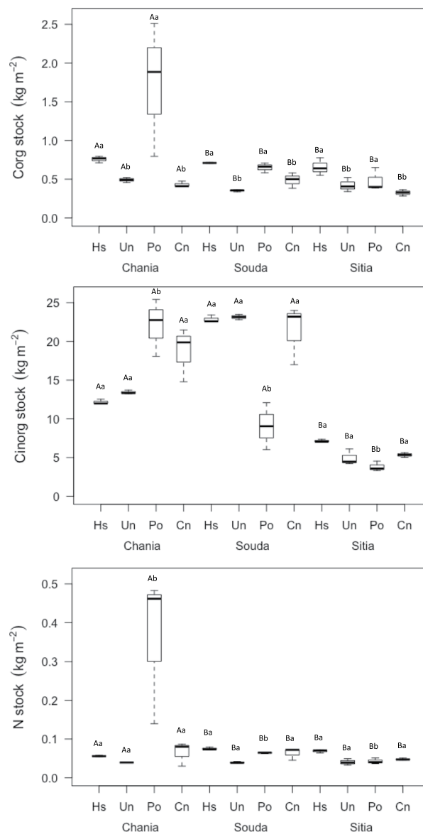
Figure 1. Box plots of organic and inorganic carbon and nitrogen stocks ( \text{kg m}^{-2} ) at each habitat of the Mediterranean Sea. Significant difference ( P < 0.05 ) between sites and habitats are given by capital and small letters, respectively.
