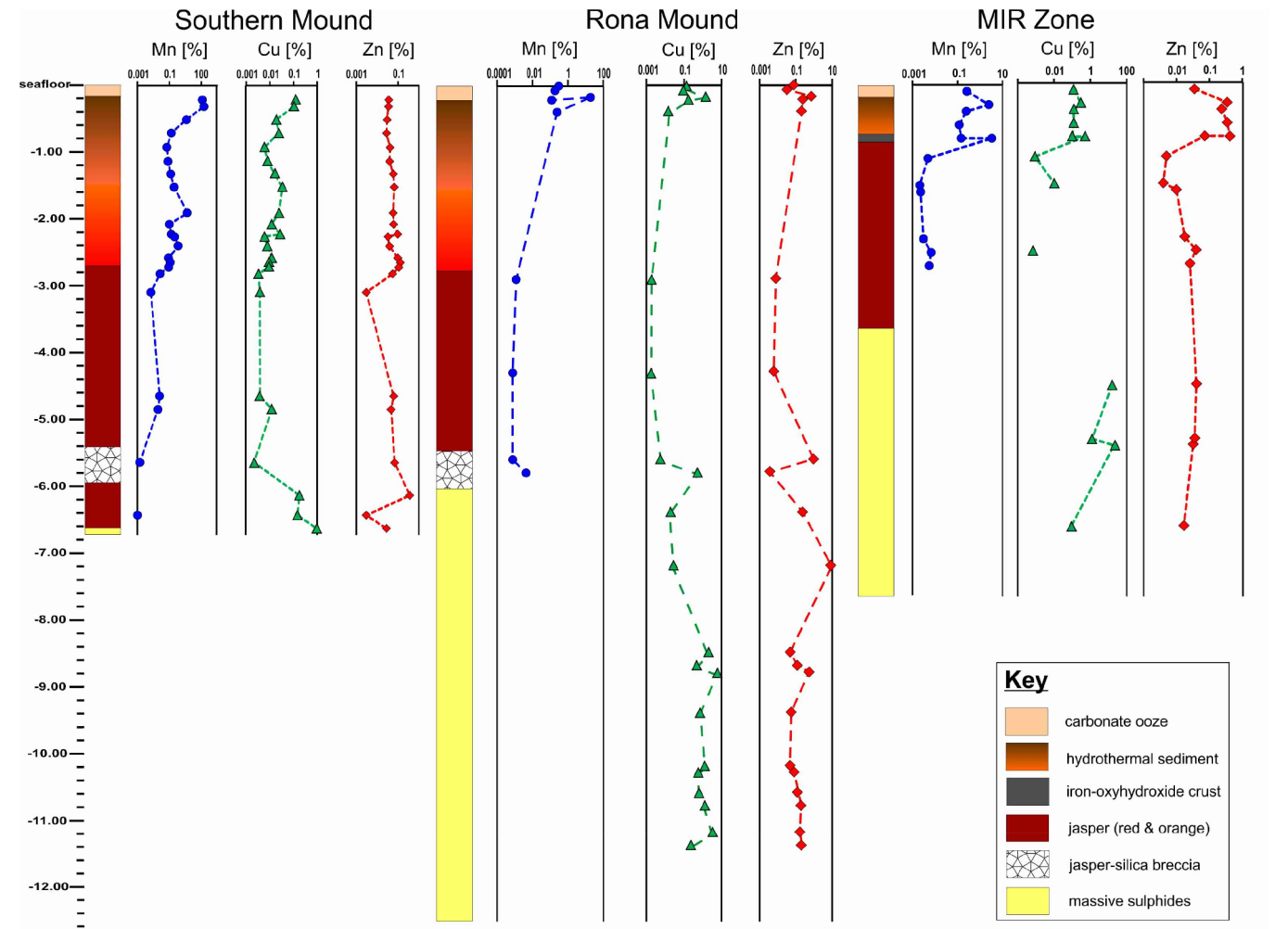
Fig. 10. Composite stratigraphy obtained for Southern Mound, Rona Mound, and the MIR Zone from coring and drilling, with downhole geochemical trends for manganese, copper and zinc. Data are from bulk samples with depths reconstructed from drilling data and core recovery (see Methods for details).
