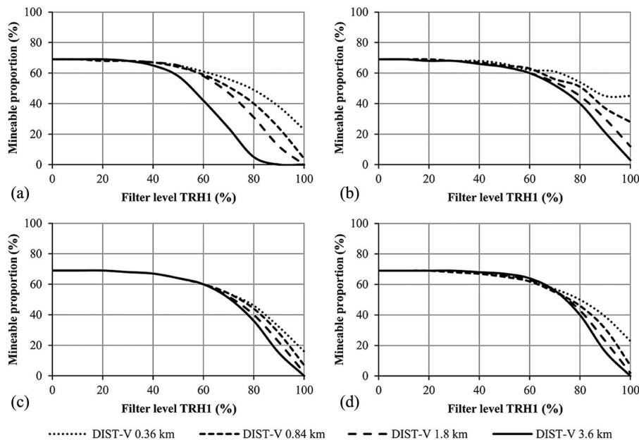
Figure 6. Potentially mineable proportion computed for the study area. (a) Radial filter. (b) Bidirectional filter. (c) Bidirectional filter with a horizontal distance of 0.36 km. (d) Mixture of a radial and bidirectional filter (for all: \vartheta = -16.5^\circ , TRH2 = TRH1, DIST-V is the vertical filter distance).
