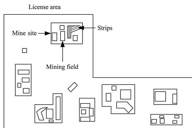
Figure 3. Schematic illustration of a mine design for SMnN. Note: SMnN, seafloor manganese nodules.
