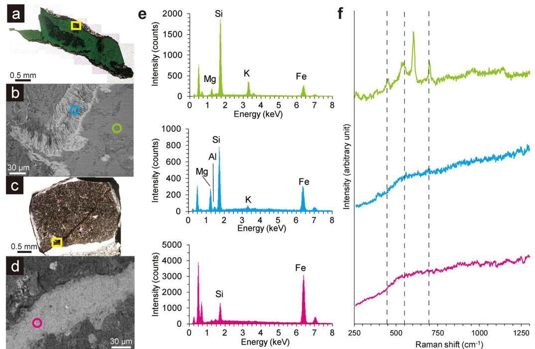
Figure 1. Spectroscopic characteristics of fractures/veins in basaltic basement at Site U1365 (104 Ma). Optical microscopy images and back-scattering electron images (BEI) from U1365E-8R4 (a,b) and U1365E-12R2 (c,d). Highlighted areas with yellow rectangles in optical microscopy images correspond to BEI images. (e) SEM-EDS spectra with colours obtained from circles with the same colours in the BEI. (f) Raman spectra obtained from the circles with the same colours in the corresponding BEI. Peak positions of three major peaks in a Raman spectrum of a celadonite standard from RRUFF are shown with dotted lines.
