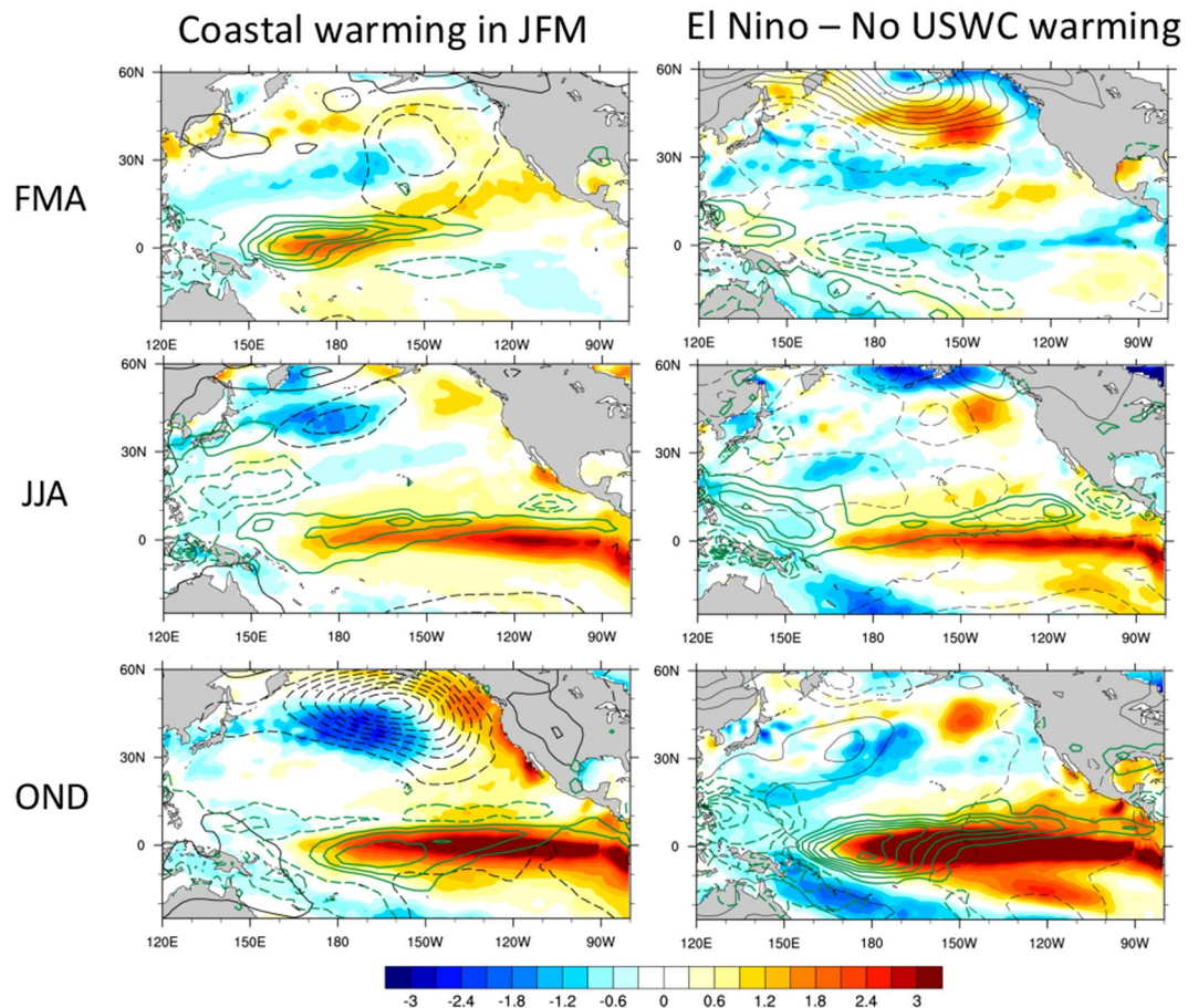
Figure 5. USWC warming vs. no-USWC warming. Comparison of the composite evolution of SST (shading), SLP (black contours, negative values dashed) and precipitation (green contours, negative values dashed) anomalies during El Niño events with no USWC warming (right panels) and for the cases of USWC warming during JFM, a season characterized by the largest USWC SST variance (left panels). El Niño events with no USWC warming were identified by requiring that the Niño3.4 index exceeds 1 standard deviation during DJF, but the SST C index is below 1 standard deviation during JFM of the same winter. The fields are displayed for the FMA, JJA and OND seasons prior to the Niño3.4 and SST C maxima. Contour intervals are 0.1 °C for SST, 0.5 mbar for SLP, and 0.5 mm/day for precipitation.
