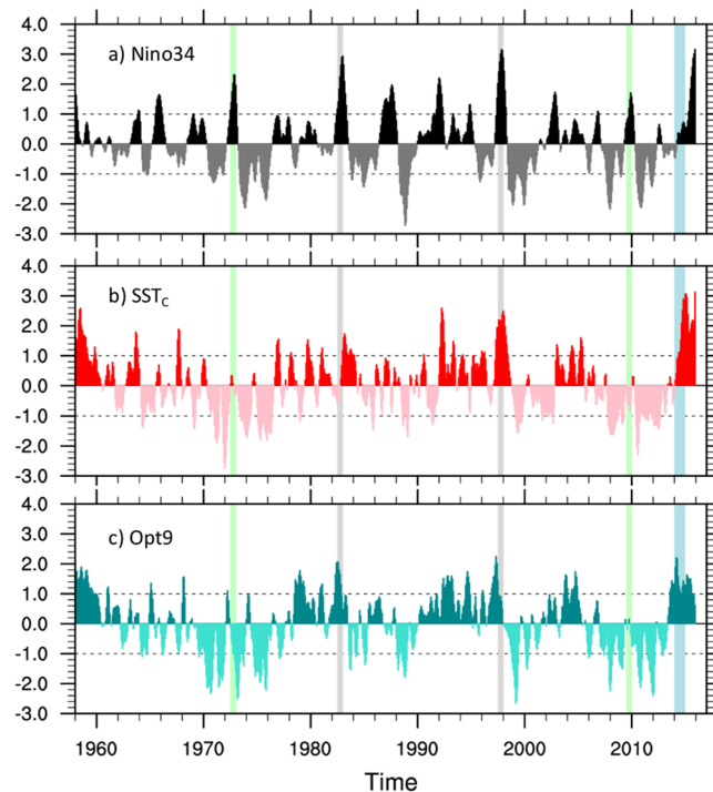
Figure 2. Comparison of relevant time series. (a) Time series of the Niño3.4 index (average SST anomaly in the region 5°S–5°N, 150°W–90°W) from January 1958 to December 2015. (b) SST anomaly index along the USWC ( SST_c ) computed as the SST anomaly averaged in the strip 30°N to 55°N and the coast to approximately 300 km offshore. (c) Index describing the evolution of the sensitivity pattern in Fig. 3a. This sensitivity pattern is obtained using equation 1 with a lead time \tau = 9 months. The associated index (Opt9) is calculated by projecting SST and SSH anomaly fields onto the sensitivity pattern. Thus, the values of Opt9 at each time correspond to the uncentered pattern correlation of the observed SST/SSH fields with the sensitivity pattern. Gray vertical bars identify two El Niño events (1982/83 and 1997/98) that were associated with large values of SST_c , light green bars indicate two El Niño events (1972/73 and 2009/10) that corresponded to very small values of SST_c , and the light blue bar highlights the 2014 case, where strong warming along the USWC was associated with small values of the Niño-3.4 index.
