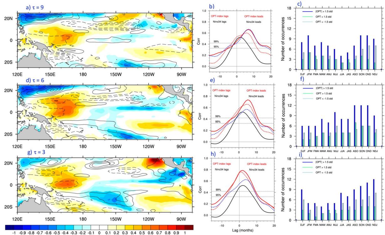
Figure 3. Sensitivity patterns. The left panels show the SST/SSH sensitivity patterns obtained for \tau = 9 (a), 6 (d) and 3 (g) months using equation (1). SST anomalies are shaded, while SSH anomalies are contoured. Units are arbitrary. SSH contour interval is 0.2. Middle panels show the lag-correlation of the indices (optimal indices) associated with the sensitivity patterns to the left with the SST_c index (red lines) for \tau = 9 (b), 6 (e) and 3 (h) months. The lag correlation obtained with the three indices is compared with the lag-correlation between the Niño3.4 index and SST_c (black line), as well as with the lag-correlations obtained using only SST in the tropical state vector (red dashed line), and using a meridionally narrower ( 15^\circ\text{S} – 15^\circ\text{N} ) tropical domain (blue dashed line). The optimal indices and the Niño3.4 index lead SST_c for positive lags and lag it for negative lags. The values of the correlations corresponding to the 95% and 99% statistical significance levels are indicated by the dotted lines. The right panels provide a measure of the seasonality of the sensitivity patterns on the left. Green bars indicate the number of times the optimal index exceeds 1.5 standard deviations (indicating a strong projection of the SST/SSH anomaly fields at that time on the corresponding sensitivity pattern) in each season, light blue bars indicate the number of times the index is less than -1.5 its standard deviation in each season, and the blue bars are the sum of the previous two cases ( |\text{OPT}| > 1.5 \text{ std} ).
