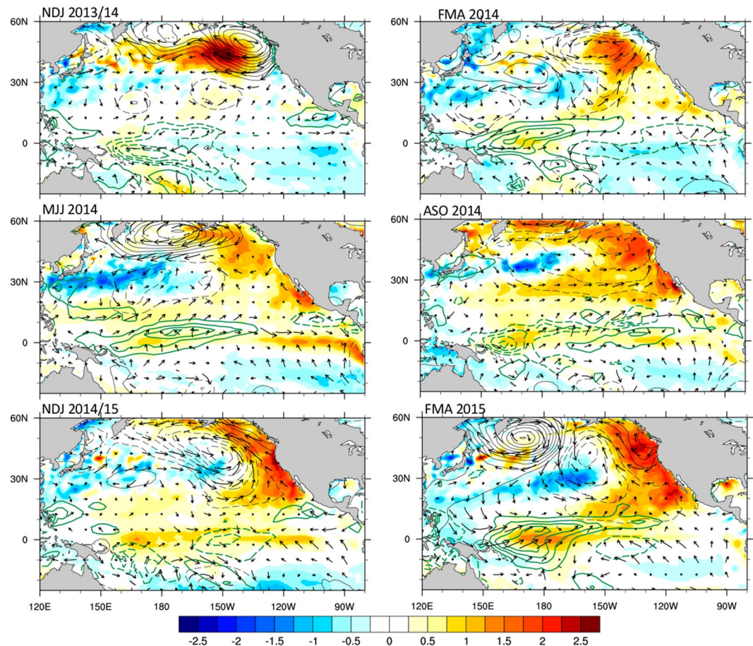
Figure 1. Northeast Pacific “marine heat wave”. Evolution of the SST (shading), SLP (black contours, negative values dashed), precipitation (green contours, negative values dashed) and surface winds (arrows) anomalies, from NDJ 2013/14 to FMA 2015. Contour intervals for SLP and precipitation are 0.8 mbar, and 0.8 mm/day, respectively. SST units are °C.
