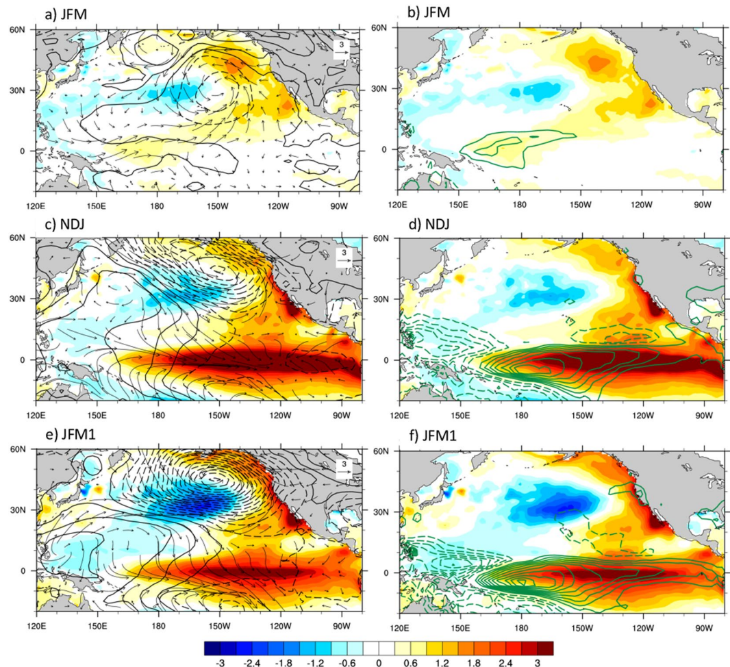
Figure 4. Composite evolution of optimal oceanic and atmospheric conditions. Composites (positive minus negative occurrences) of SST (shading), SLP (contours) and surface wind (arrows) anomalies on the left, and SST (shading) and precipitation (green contours) anomalies on the right, based on the sensitivity pattern obtained for \tau = 3 months (Fig. 3g). The largest number of occurrences of this pattern is in NDJ. Composites for this season are shown in (c) and (d), while (a) and (b) show the composites for the preceding JFM, and (e) and (f) the composites for the following JFM seasons. Contour intervals are 0.3 °C for SST, 1 mbar for SLP, and 1 mm/day for precipitation.
