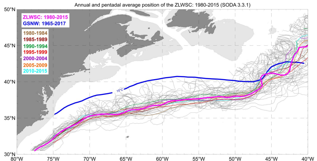
Figure 3. Positions of the zero line of annually averaged wind stress curl (ZLWSC) for each year from 1980 to 2015 (grey lines). The bold blue line shows the GSNW position averaged over all years from 1965 to 2017 for the GS area (same as in Fig. 2). Pentadal ZLWSC positions from 1980 to 2015 shown as colored lines. The ZLWSC averaged over all pentads is shown by the bold magenta line. Wind stress data are from SODA v3.3.1 re-analyses. The ZLWSC is shown only above the GS jet region, with the areas adjacent to the East Coast and the Grand Banks excluded.
