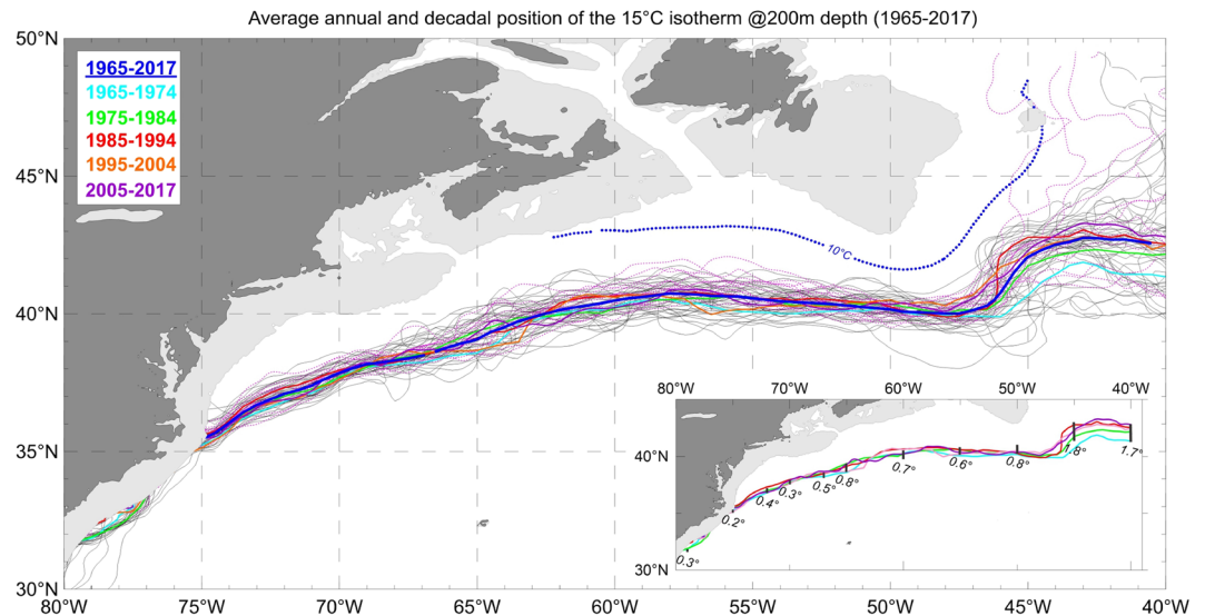
Figure 2. The ensemble of the annually averaged positions of the 15 °C isotherm at 200 m depth (GSNW) for each year (1965–2004: grey lines; 2005–2017: dotted magenta lines), five decadal-annual positions of the GSNW (five colored lines), and the 1965–2017 average GSNW position (bold blue line). The 10 °C isotherm at 200 m depth (blue dotted line) illustrates the North Atlantic Current veering northward from the GSNW branch that aligns with the Azores Current (see the scheme in Fig. 1). The standard deviations (degrees of latitude) are shown by bars with numbers in the insert together with decadal-annual positions of the GSNW (five bold colored lines).
