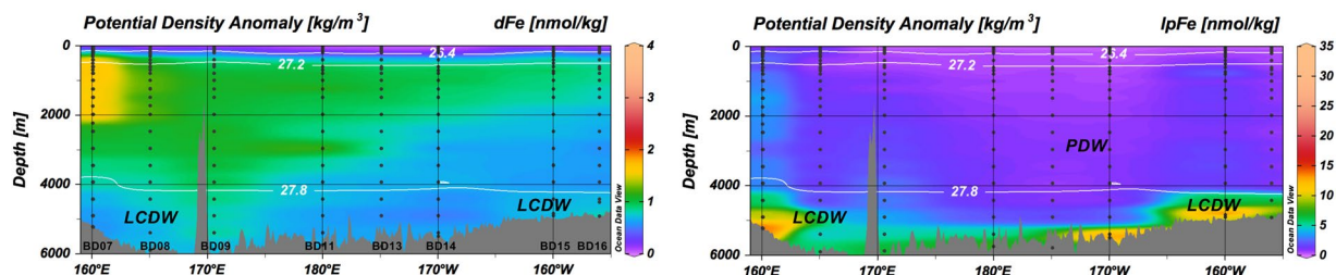
Figure 1. Full-depth sectional distribution of dFe and lpFe along 160°W, 165°E, and 47°N. The potential density isolines of 26.4 and 27.2 represent the upper and lower boundaries of the North Pacific Intermediate Water (NPIW), and those of 27.8 represent the upper boundary of the Lower Circumpolar Deep Water (LCDW). EqPIW: Equatorial Pacific Intermediate Water; UCDW: Upper Circumpolar Deep Water; PDW: Pacific Deep Water.
