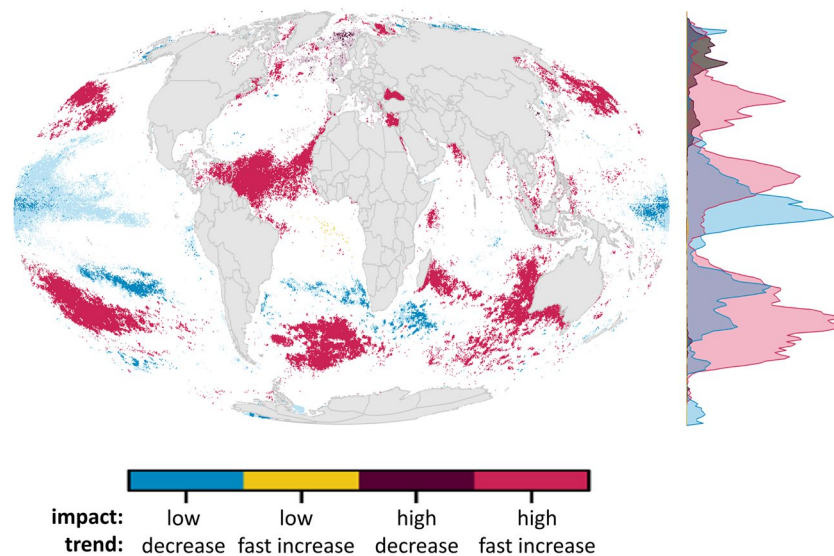
Figure 2. Overlap of extreme impact (high, low) and trend (fast increase, decrease) in cumulative impacts. Regions of low ( <20^{\text{th}} quantile) and high ( >80^{\text{th}} quantile) cumulative impact in 2013 were combined with regions where annual cumulative impacts were decreasing (trend \leq 0 , lighter colors represent non-significant trends) or quickly increasing (trend >80^{\text{th}} global quantile, corresponding to a slope estimate of 0.085, all significant trends). Trend estimates were calculated using a linear regression model from 2003–2013 cumulative human impacts. Density plot on right shows the distribution of values across latitude.
