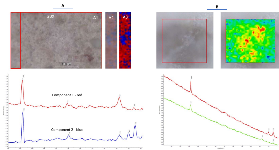
Figure 4. Raman spectroscopic imaging. (A) Raman Image and Multivariate Curve Resolution (MCR) analysis of powder sample. Light (A1) and Multivariate Curve Resolution (MCR) Raman (A2, A3) images of sample. The 2 components of MCR analysis corresponding to red and blue areas in image and showing, respectively, Raman peaks of Calcite (1086, 711, 284 and 158 \text{cm}^{-1} ) and Aragonite (1082, 700, 279, 205 and 150 \text{cm}^{-1} ). Blue areas corresponding to aragonite occupy about 29% of the total area of sample. (B) Detection of minerals in the skeleton. Representative averaged Raman spectra from red (aragonites) and green (calcites) areas of the image, respectively, showing a peak at 206 \text{cm}^{-1} and shift of most intense peaks from 1087 to 1083 \text{cm}^{-1} . This provides evidence for the presence of aragonite in red areas. Spectra are shown on a common scale.
