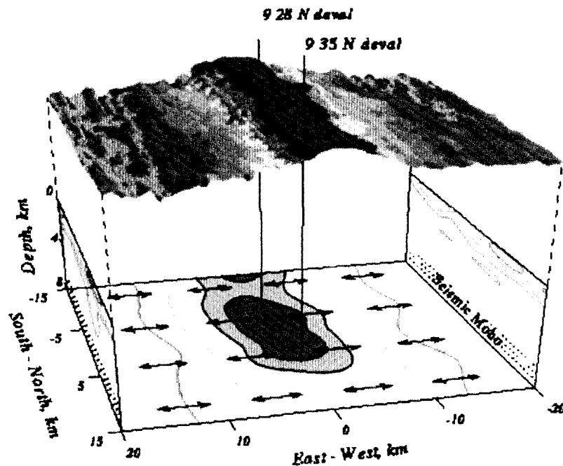
FIGURE 3 Seafloor bathymetry and results of seismic tomographic imaging on the East Pacific Rise, at 9^{\circ}30'N (from the TIERRA project, http://www.csi.uoregon.edu/projects/tierra/tierra_overview.html and Dunn et al. 2000). Seismic tomography samples the Earth's interior via earthquake waves recorded by seismic instruments. Velocity anomalies are shown at a 0.2 km/s contour intervals, and arrows in the horizontal plane indicate orientation of the fast axis of anisotropy (properties such as temperature, strain, and melt varying in different directions). "Deval" signifies deviation in axial linearity, which may affect the distribution of magma on the seafloor along the axis of the rise.
