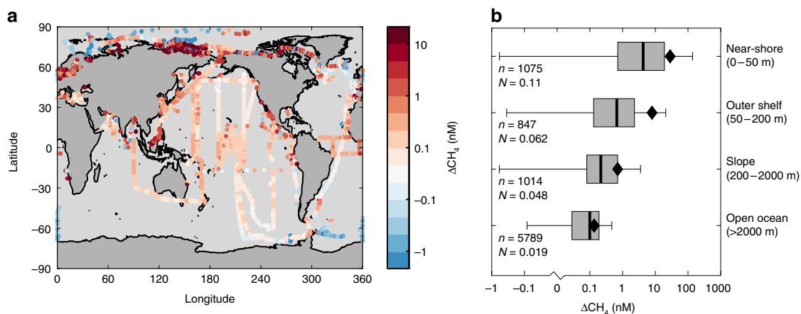
Fig. 1 Global \Delta\text{CH}_4 climatology. a Annual-mean \Delta\text{CH}_4 , computed after binning all data into 0.25^\circ \times 0.25^\circ monthly climatology. Data points are drawn larger than the grid cells for clarity. b Probability distributions of observed \Delta\text{CH}_4 , grouped into four bathymetric regions (see also Supplementary Fig. 2). Boxes span the interquartile range, with black line at median. Black diamonds are mean values, and whiskers span the 5–95th percentiles. Number of datapoints ( n ) and data density per 10^9 \text{ m}^2 ( N ) after binning are listed
