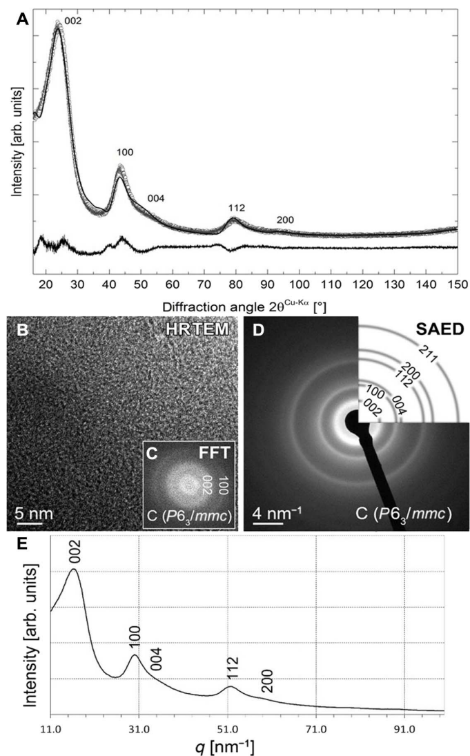
Fig. 2. Identification of carbonized spongin as turbostratic graphite. XRD analysis of spongin carbonized at 1200°C. (A) Circles, measured data; solid line, calculation according to the method described (25) and values given in table S1; bottom line, difference between measured and calculated intensities. Labels are the diffraction indices hkl . (B) HRTEM image with corresponding indexed FFT (C). (D) SAED pattern for carbonized spongin and corresponding 1D intensity distribution (E) as the sum of intensities along the diffraction rings.
