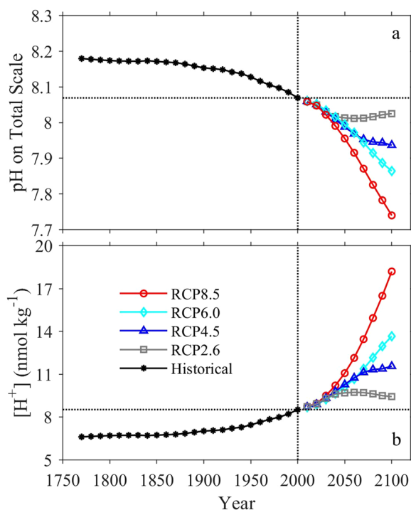
Figure 5. Long-term change of global surface ocean pH T and ocean acidity. Panel a, the globally and annually-averaged surface ocean pH T from 1770 to 2100. Panel b, the change of ocean acidity (hydrogen ion activity, [H + ], 1 nmol kg -1 = 1 × 10 -9 mol kg -1 ) over the same period.
