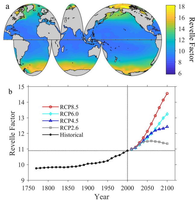
Figure 4. Spatial and temporal distributions of global surface ocean Revelle Factor. Panel a, the spatial distribution of annually-averaged Revelle Factor adjusted for the year 2000 in the global surface ocean. Panel b, the long-term change of the globally and annually-averaged surface Revelle Factor from 1770 to 2100 under all Representative Concentrations Pathway (RCP) scenarios.
