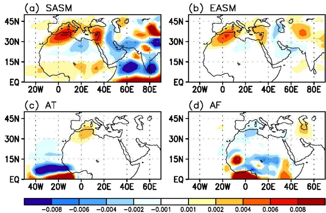
Figure 2. Simulated descending motion anomalies in response to each forcing. Middle troposphere ( \sigma = 0.550 ) omega anomalies (shading; \text{Pa s}^{-1} ) averaged over 25–29 days of model simulation in response to the (a) SASM, (b) EASM, (c) Atlantic, and (d) African forcings. Maps were generated using GrADS version 1.9b4 ( http://grads.iges.org/grads/ ).
