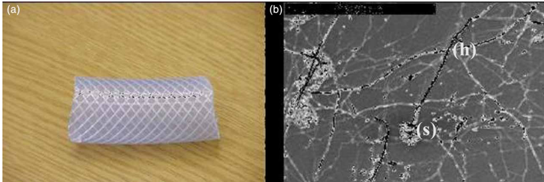
Figure 4 | (a) Excised piece of a new product water replacement hose showing lack of growth by the naked eye and (b) SEM of the internal surface showing fungal hyphae (h) and spores (s).
