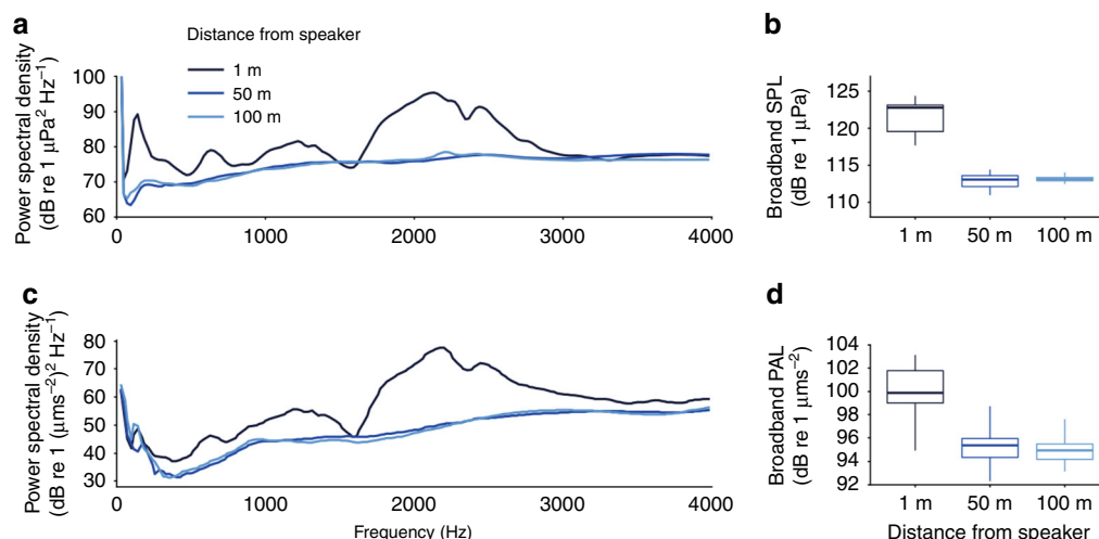
Fig. 6 Recordings of reef-sound playback taken at 1, 50 and 100 m from the loudspeaker. Shown are: a power spectral densities from a single full-night recording taken in sound-pressure; b boxplots of total received broadband (10–4000 Hz) sound pressure level (SPL) from evenly spaced 2-min sub-samples throughout the night ( n = 20 ); c power spectral densities similar to a but showing particle acceleration; and d boxplots of total received broadband (10–4000 Hz) particle-acceleration levels (PAL) similar to b . Boxplots in b and d represent medians (central lines), interquartile ranges (boxes), and 95% ranges (whiskers).
