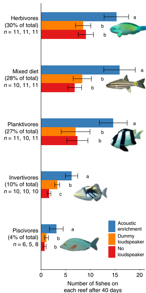
Fig. 2 Effects of acoustic enrichment on different trophic groups. Mean \pm SE juvenile fish abundance in different trophic guilds on experimental patch reefs. Y-axis labels give the proportion of all fishes and the frequency of occurrence (number of populated reefs in each loudspeaker treatment) represented by each trophic guild. Mixed-effects models revealed significant effects of loudspeaker treatment in all five trophic guilds; different letters associated with boxplots represent significant differences in post-hoc Tukey's HSD tests (Supplementary Table 1). Images of fish are taken from the Lizard Island Field Guide ( liff.australianmuseum.net.au ), licensed under the Creative Commons Attribution 3.0 License ( creativecommons.org/licenses/by/3.0/ ).
