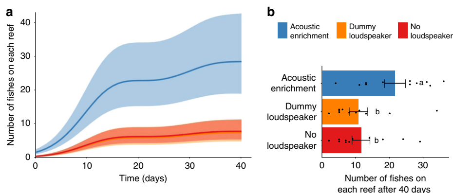
Fig. 1 Effect of acoustic enrichment on damselfish community development. a Outputs from a generalised additive mixed model, modelling number of juvenile damselfish per reef (mean \pm SE) over time based on repeated surveys; orange and red lines and ribbons are almost completely overlapping. b Raw count data of number of juvenile damselfish per reef (mean \pm SE) from surveys undertaken after 40 days. Different letters associated with bars represent significant differences in post-hoc Tukey's HSD tests, following a significant effect of loudspeaker treatment in a generalised linear mixed model (see Supplementary Table 1).
