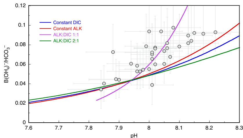
Fig. 3 Sensitivity of pH vs. [B(OH)_4^-]/[HCO_3^-]_{sw} relationship to DIC and ALK. pH estimates derived from boron isotope reconstructions 35 and ad hoc B/Ca- B(OH)_4^-/DIC and B/Ca- [B(OH)_4^-]/[HCO_3^-]_{sw} calibrations (see Methods) are plotted for a range of scenarios with changes in the dissolved inorganic carbon (DIC) and alkalinity (ALK) inventory. Blue and red line indicate scenarios with constant DIC and ALK, respectively. Purple and green lines indicate changes with a ALK:DIC ratio of 1:1 and 2:1. We plot one \delta^{11}B_{sw} 35,66 (G17) scenario to highlight the overall relationships present and provide full carbonate system estimates in the Methods. Monte Carlo uncertainty estimates (95% CI) are plotted for pH 35 and [B(OH)_4^-]/[HCO_3^-]_{sw} estimates.
