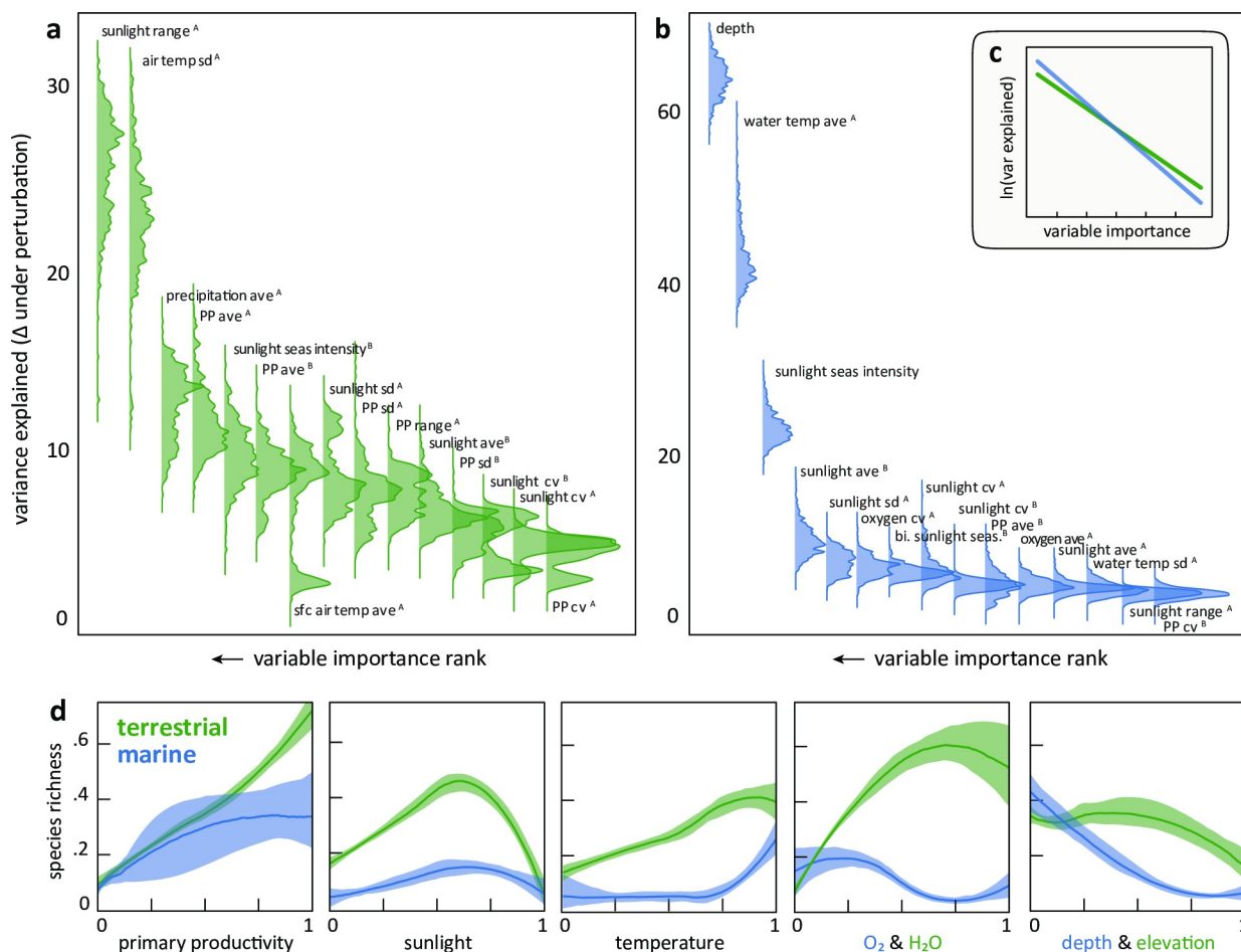
Fig 2. Environmental drivers of species richness in marine and terrestrial domains. The ranked importance of the top 15 environmental variables in the (a) terrestrial and (b) marine ANNs. Bootstrapped driver variable importance plots display the densities of change in explained variance made when perturbing individual model factors. The process is repeated 500 times with a random subset of the data on which a new ANN model is trained, generating a robust importance ranking by allowing multiple weight matrices to be evaluated as to how they learn the driver-richness relationship. On the variable labels, “A” is measured within year, “B” is between years. (c) Inset plot shows these same relationships on a log-linear scale, highlighting the steeper decline of variable importance and therefore greater effect of fewer variables in marine systems. (d) Pairwise plots showing the effects from a subset of individual drivers on species richness. To alleviate overplotting, graphs display the median ensemble (with 95% quantiles) of 100 local regression models fit from resamples of the global dataset. For (d) all variables are annual means and rescaled to 0–1 without further transformation. Similar factors are plotted when the same do not exist in both domains. Supporting information provide the full list of all modelled variables and their explanation.
