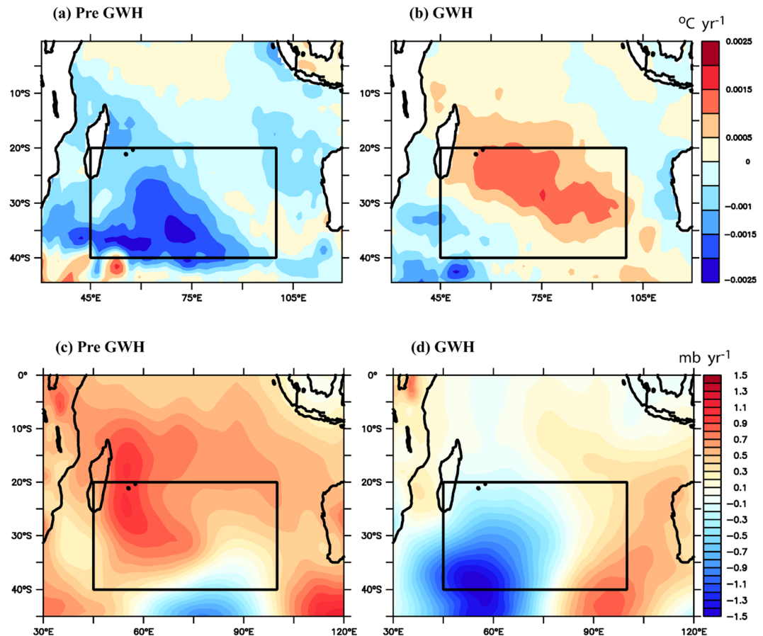
Figure 4. Spatial pattern of trend of (a) SST during preGWH, (b) SST during GWH, (c) MSLP during preGWH, (d) MSLP during GWH.
