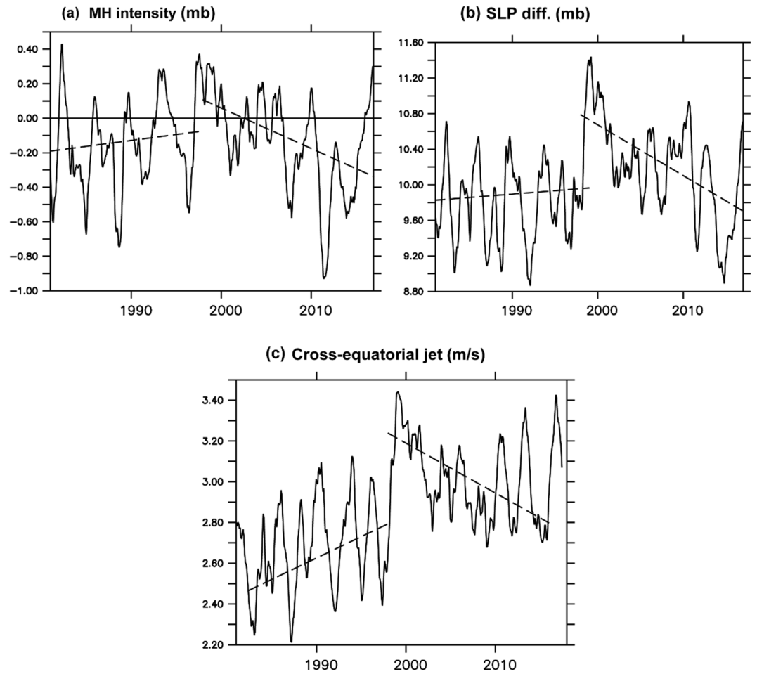
Figure 5. (a) Time series of monthly mean SLP, (b) SLP difference between the MH [45°E–100°E and 20°S–40°S] and the Indian landmass [45°E–100°E and 10°N–35°N], (c) Cross-equatorial winds [37.5°E–60°E and 5°S–5°N]. All trends are significant above a 95% confidence level.
