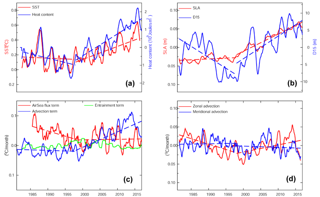
Figure 2. Monthly mean anomalies of (a) SST (red) and heat content (blue), (b) sea level (red), (c) mixed layer budget terms (Air-sea flux term - red, Advection term - blue, Entrainment term - green), (d) zonal (red) and meridional (blue) component of the advection term in the Mascarene High region [20°S–40°S & 45°E–100°E]. The dashed lines represent the trend line. All trends are significant above a 95% confidence level.
