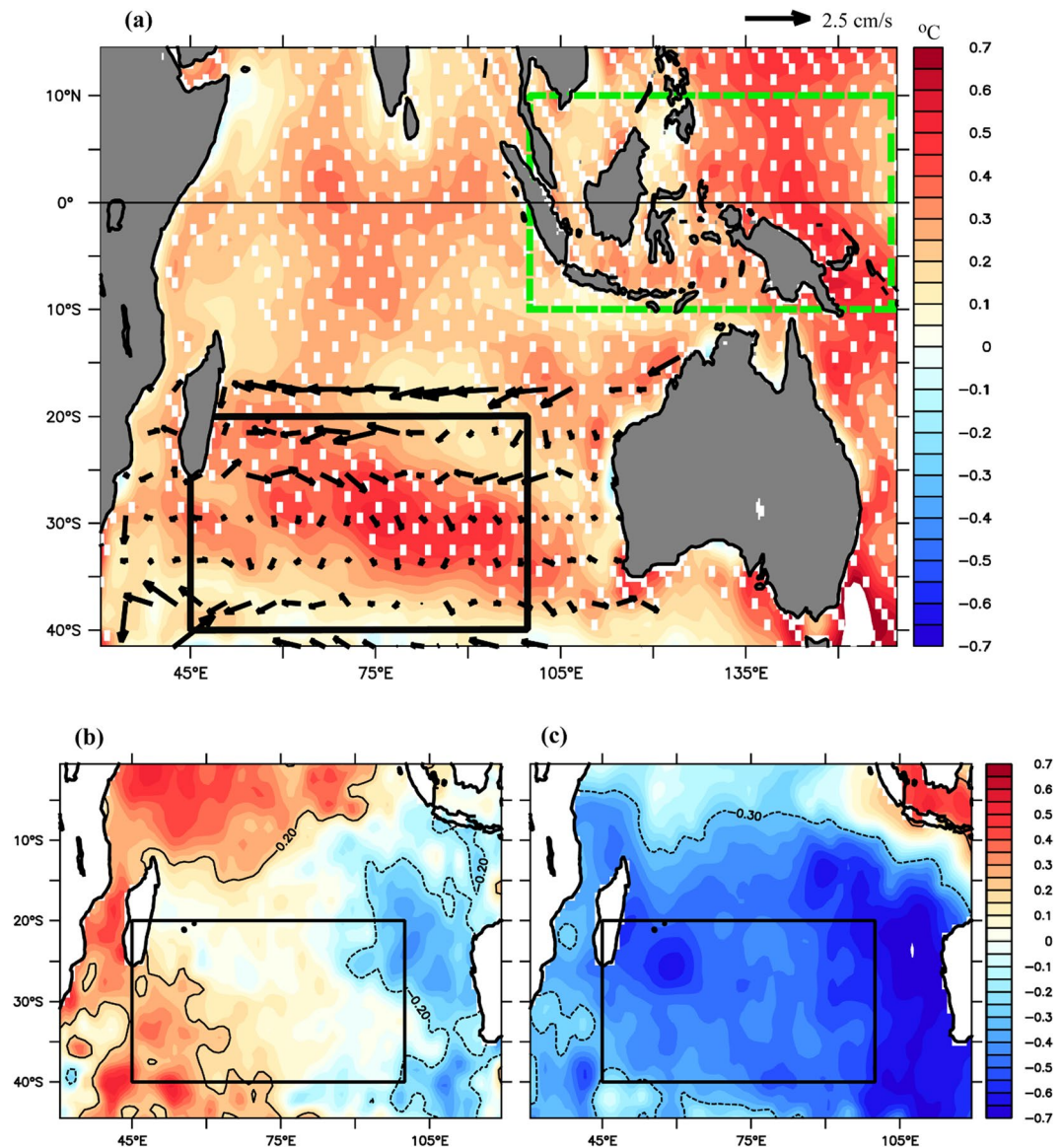
Figure 3. (a) SST difference between the GWH (1998–2016) and preGWH (1981–1997) overlaid with the current anomaly (GWH-PreGWH) of upper 100 m. White dots represent the SST anomaly above 90% significance level (b), Correlation between MH intensity and SST during the preGWH and (c), Correlation between MH intensity and SST during the GWH. The dashed/solid contour indicates 90% significance level. The black rectangle in (a–c) represent the MH region, and the dashed green rectangle in (a) represents the western Pacific region.
