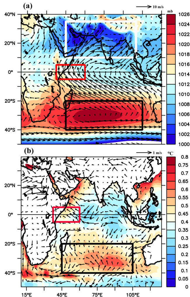
Figure 1. (a) Spatial pattern of Mean Sea Level Pressure overlaid with climatological winds (10 m) during the boreal summer (June–September), (b) Standard deviation of annual mean sea surface temperature overlaid with wind anomaly (GWH-preGWH). In Figure (a and b), the black rectangle in the southern hemisphere indicate the MH region [45°E–100°E and 20°S–40°S], the red rectangle indicates the cross-equatorial winds [37.5°E–60°E and 5°S–5°N]. In (a), the white rectangle indicates the Indian landmass [45°E–100°E and 10°N–35°N], where the SLP difference was plotted in Fig. 5b. SLP and Winds were taken from ERA-interim, and SST was taken from OISST.
