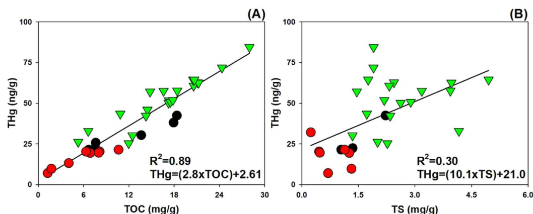
Figure 3. Relationships between TOC (A), TS (B) and THg concentrations of the surface sediments in the Svalbard fjords that were studied.
