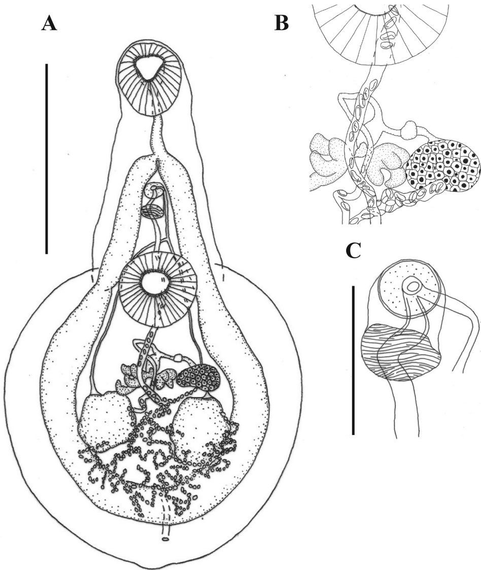
Figure 4. Line drawings of the 532 CHCM-voucher of Xystretrum solidum from the urinary bladder of Spheroideus testudineus A whole specimen (ventral view) B details of reproductive organs C details of genital atrium. Scale bars: 1000 \mu\text{m} ( A ); 250 \mu\text{m} ( B–D ).
