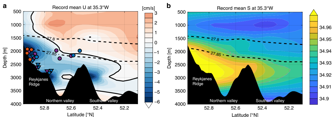
Fig. 1 Vertical sections across the Charlie–Gibbs Fracture Zone (–35.3°W). a Zonal mean velocity from mooring observations. Superimposed are the 21 RAFOS floats' positions while crossing through/nearby the section. Triangles show release locations for nine floats in the northern valley and circles show locations of the remaining 12 floats while passing through/nearby the section. Marker color indicates the pathway each float took: blue for west-northwestward pathway; purple for southward pathway; and orange for eastward pathway. b Mean salinity from the same source. On both plots, dashed black contours show isopycnals.
