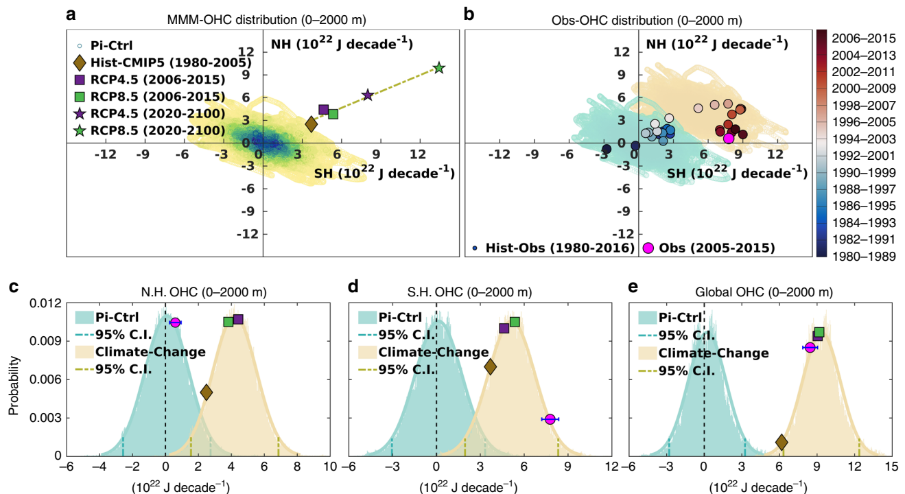
Fig. 3 Probabilistic analysis of the ocean heat content anomaly trend. Distribution of the linear trend of the OHC anomaly ( 10^{22} \text{ J decade}^{-1} ) for the depth of 0–2000 m for Northern (NH) and Southern Hemisphere (SH) from (a) multi model ensemble (MME) of pre-industrial control (Pi-Ctrl) simulation (cloud), with the multi model mean (MMM) trend from the historical (Hist-CMIP5, brown diamond, 1980–2005), RCP 4.5 (purple square 2006–2015; purple star 2020–2100) and RCP 8.5 (green square 2006–2015; green star 2020–2100) simulation, and the least square fit line passing through these points to represent the direction of climate change (b) the green cloud is the same as shown in (a) and the orange cloud is the represent the climate change signal in the direction of the best fit line as shown in (a), Observed trend over the period of 2005–2015 (Obs, pink circle) along with the trajectory (scatter dots) of the 10-year running trends from the long-term observations over the period of 1980–2016 (Hist-Obs). c Probability distribution curve for the northern hemisphere's internal variability (green cloud in (b)) and climate change (orange cloud in (b)) with the OHC trend from observations (pink circle with the error bar of 95% confidence intervals from two-sided student's t-test, 2005–2015), MMM of historical (brown diamond, 1980–2005), RCP 4.5 (purple square, 2006–2015) and RCP 8.5 (green square, 2006–2015) simulations. d, e Same as (c) but for the Southern Hemisphere and the Global Ocean respectively. The 95% confidence interval for the probability distribution curves is derived from the 2-sigma limits for the gaussian distribution of OHC trend.
