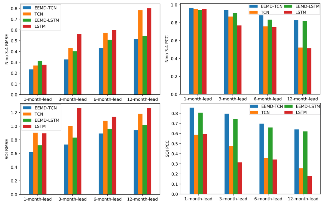
Figure 12. RMSE and PCC comparison of predicted and actual values of Niño 3.4 index and SOI obtained using the TCN, EEMD-TCN, LSTM, and EEMD-LSTM methods.
