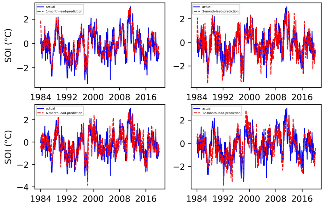
Figure 11. EEMD-LSTM-based SOI predicted and actual value curves.
