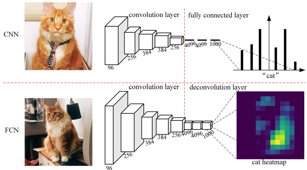
Figure 13. The difference between the CNN and FCN (the transforming of fully connected layers into convolutional layers by an FCN enables a classification net to output a heatmap).
