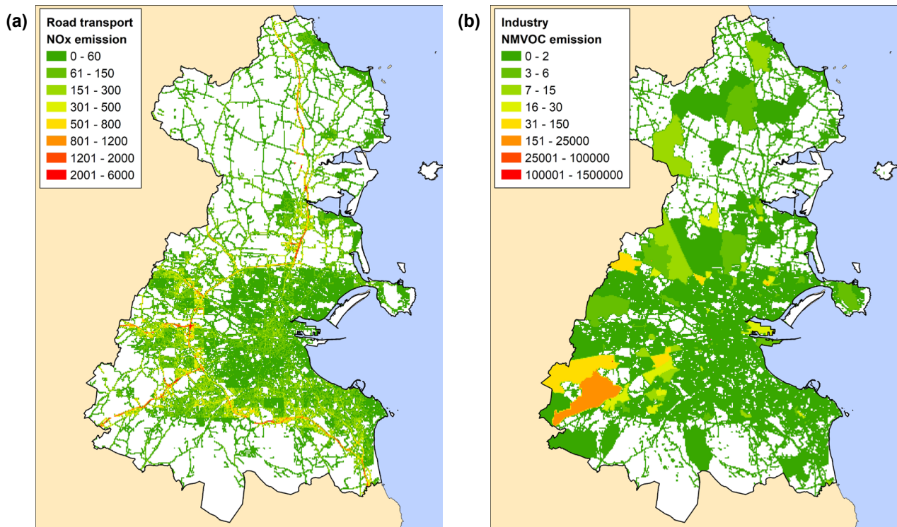
Figure 3.7. Spatial emission maps for Dublin for (a) NO x from road transport and (b) NMVOCs from industry.
