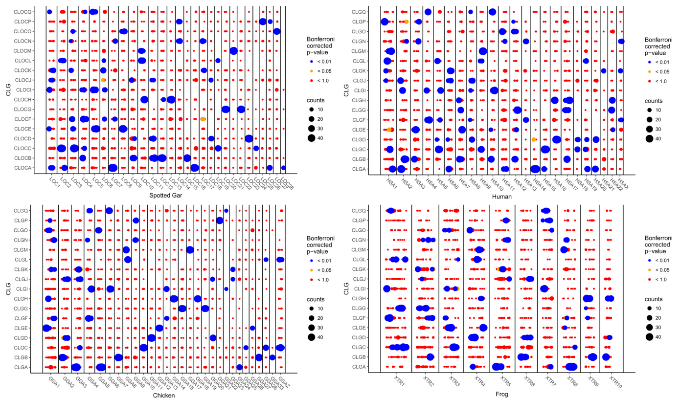
Extended Data Fig. 7 | Oxford grid showing associations between 50 gene segments of bony vertebrate chromosomes and chordate linkage groups (CLGs). Given the evident localization of orthologs along bony vertebrate chromosomes shown in the ‘Oxford’ dotplots of Fig. 1 and Extended Data Figs. 2 and 3, we assessed the significance of associations between sub-chromosomal regions and the chordate linkage groups. Each vertebrate chromosome was divided into overlapping 50 gene windows (offset by 25 genes). Only 6,843 genes with amphioxus-bony vertebrate mutual best hits are used. Circle areas are proportional to the number of orthologous genes for each chromosome-CLG pair, and the color indicates the significance of the association relative to a null model in which the position of the orthologous genes are randomly shuffled. Comparing Extended Data Figs. 6 and 7 shows additional significant associations that are missed based on whole chromosome analyses.
