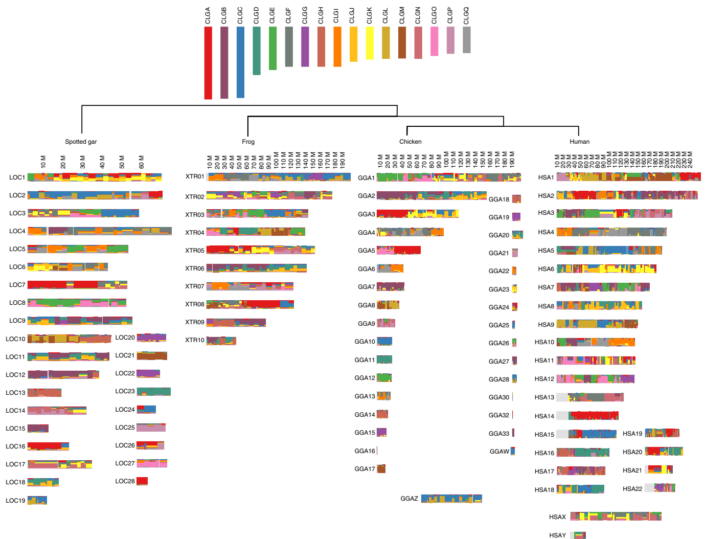
Fig. 2 | Contributions of the 17 ancestral CLGs to contemporary vertebrate genomes. The CLG ancestries of four jawed vertebrate genomes are shown by the local fraction of genes that are derived from each CLG, in windows of approximately 20 genes (see Methods). Note that, in contrast with Fig. 1, the chromosomal position is shown as physical coordinates (that is, base pairs), so area is not proportional to gene number. Colours are the same as in Fig. 1. The statistical significance of the associations between CLGs and vertebrate chromosomes is reported in Fig. 3.
