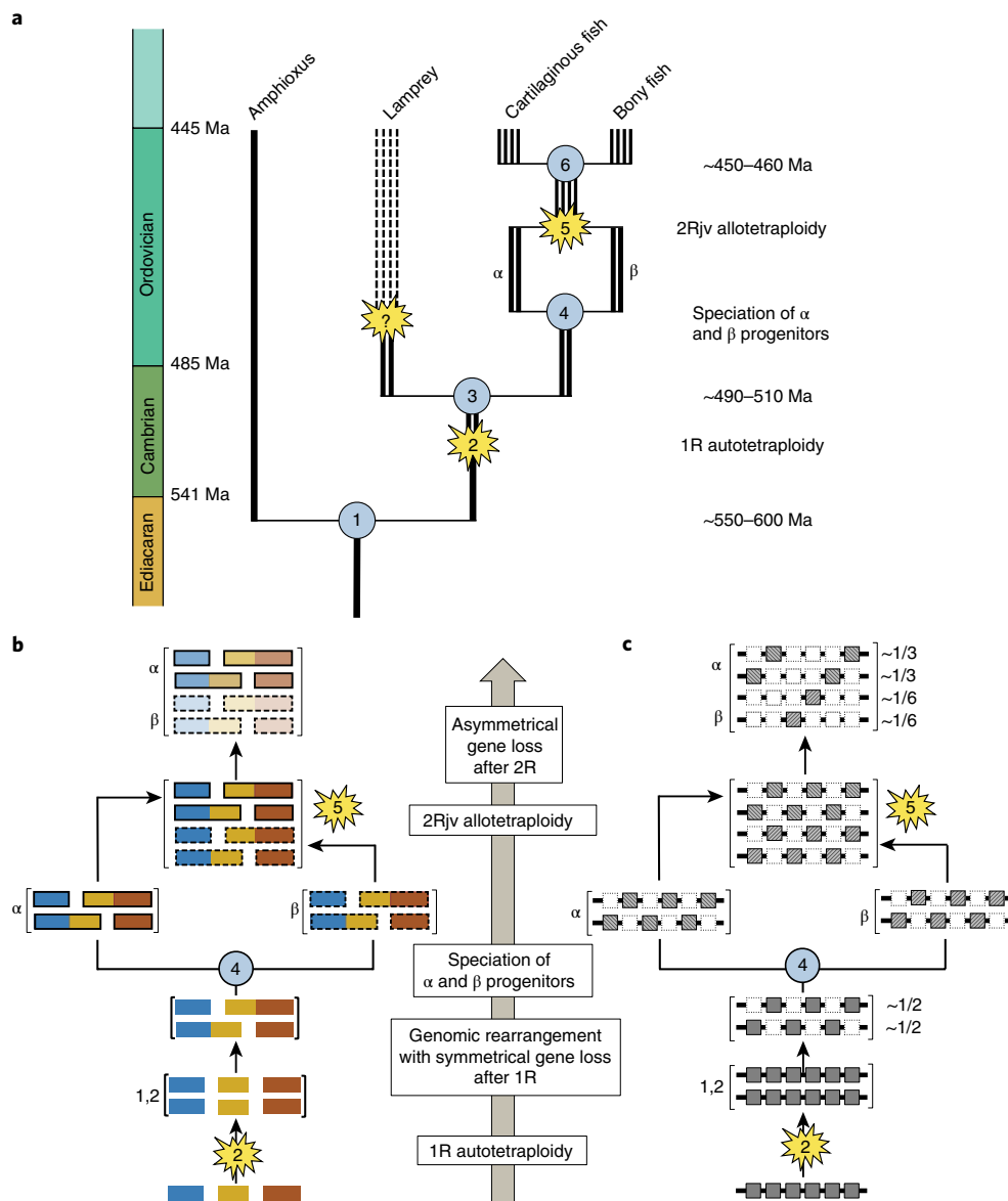
Fig. 5 | Auto- then allotetraploidy scenario for vertebrate evolution. Schematic of the auto- then allotetraploidy scenario described in the main text. a , Each line represents a chromosomal lineage. Single lines represent diploids, paired lines represent tetraploids, and so on, relative to the ancestral chordate chromosome complement. Dashed lines later in the lamprey lineage reflect one or more additional genomic duplications. Labelled nodes: (1) divergence of amphioxus and vertebrates (last common chordate ancestor); (2) 1R autotetraploidy, resulting in genome doubling; (3) divergence of (tetraploid) lamprey and gnathostome progenitor lineages; (4) speciation of palaeotetraploid gnathostome progenitors; (5) 2Rjv allotetraploidy, in which palaeotetraploid gnathostome progenitors hybridize to form the crown gnathostome lineage, which is quadrupled relative to the chordate ancestor; (6) divergence of extant jawed vertebrate lineages. The question mark indicates one or more additional duplication(s) that may have occurred in the lamprey lineage. b , Schematic showing the evolution of three ancestral CLGs. Relevant nodes are labelled as in a . Bold and dashed boundaries around chromosomes in the \alpha and \beta lineages, respectively, represent divergences that accumulate in each lineage. Differential shading after node 5 indicates subsequent gene loss. c , Schematic of the evolutionary history of six linked chordate genes through vertebrate duplications. Gene loss is symmetrical after autotetraploidy (node 2) but asymmetrical after allotetraploidy (node 5). For simplicity in this diagram, gene order changes are not shown. Cross-hatching indicates independent differentiation in \alpha and \beta lineages. Empty dashed boxes follow the fate of lost genes.
