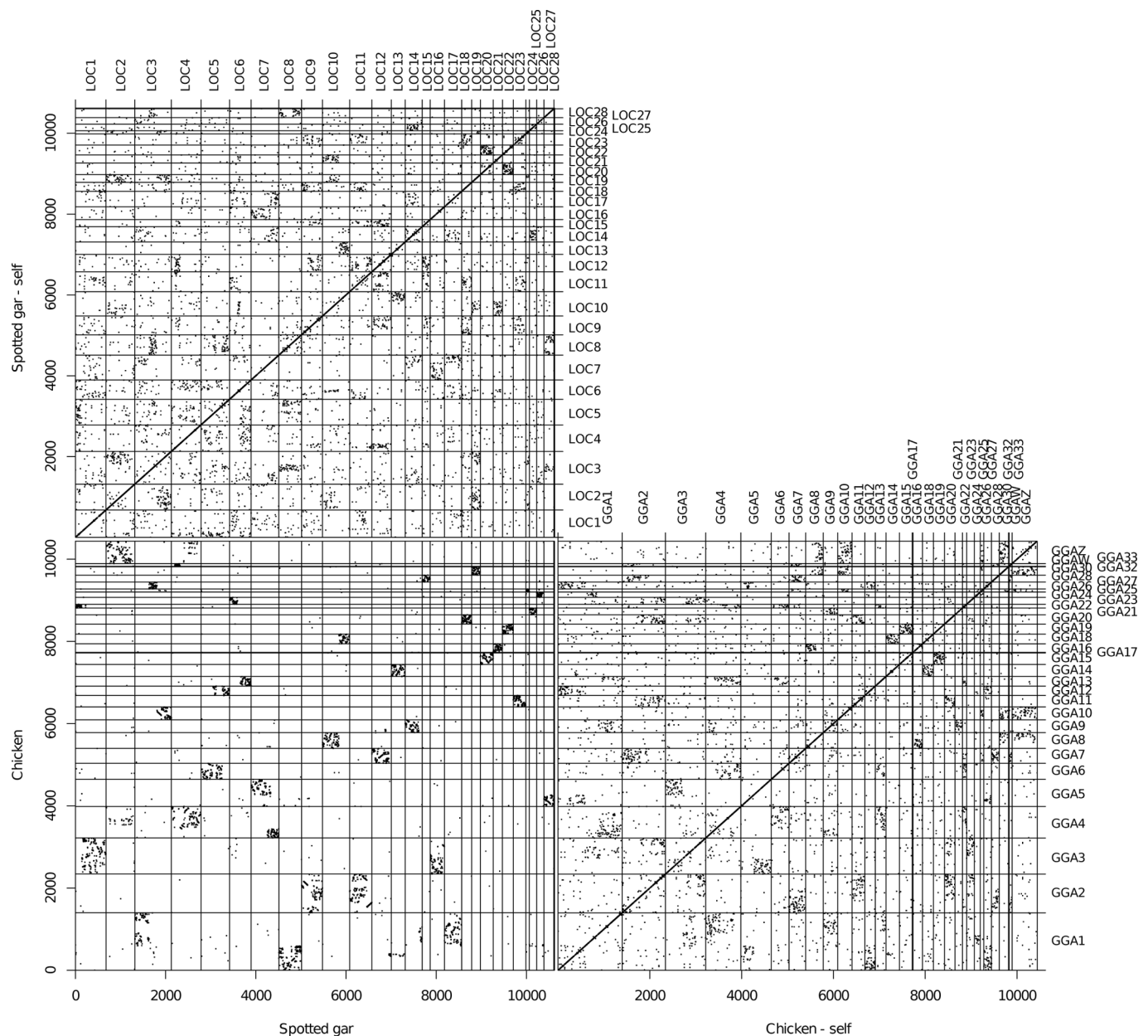
Extended Data Fig. 5 | Chicken-spotted gar orthologs and paralogs. “Oxford” dotpot between chicken ( Gallus gallus , GGA) and spotted gar ( Lepisosteus oculatus , LOC). Dots in the lower left corner represent mutual best hits between chicken and spotted gar, showing the clear orthologous blocks conserved synteny that allows chicken and spotted gar chromosome segments to be placed in correspondence with each other. Upper left and lower right show intra-genomic non-self best hits that identify paralogous regions within the chicken and spotted gar genome, respectively. Paralogous chromosomal regions share the same chordate linkage group ancestry, but arose through duplication.
