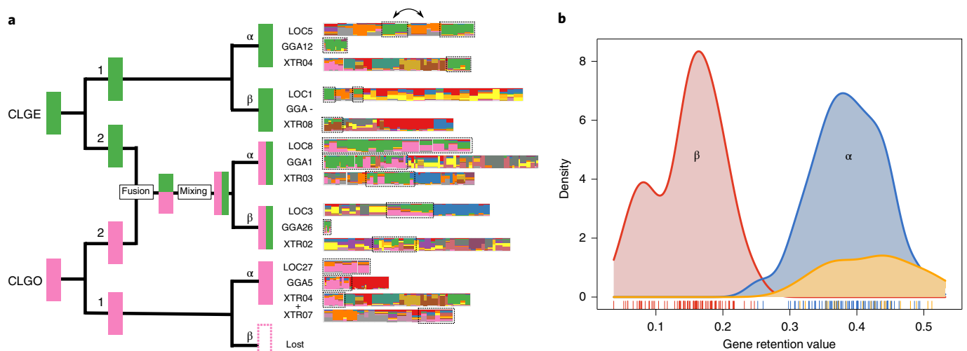
Fig. 4 | Duplications, fusions and mixing in bony vertebrates. a , Right: chromosomal descendants of CLGE (green) and CLGO (pink) are organized into five groups. Each chromosome is represented as in Fig. 2, with corresponding segments outlined by black dotted rectangles. The double-headed arrow indicates probable inversion that separated two CLG blocks. Within each group, segments with the CLGE and/or CLGO ancestry are orthologous among the chicken, gar and frog, and groups are paralogous to each other. Note that the frog chromosome XTR4 has distinct CLGE and CLGO segments with distinct ancestry (see Supplementary Note 6). Left: cladogram showing the most parsimonious evolutionary history leading to these vertebrate chromosomes, starting from CLGE and CLGO ancestors. This includes an early duplication (producing copies labelled 1 and 2), a fusion and subsequent mixing, and then a second duplication (producing copies labelled \alpha and \beta ). The CLGO-1 \beta copy was not found, as indicated by a dashed pink rectangle. CLGE-1 \beta was not found in chicken, as indicated by the dash. CLGO-1 \alpha was found split across XTR04 and XTR07, as indicated by the plus sign. b , Distribution of gene retention for the \alpha and \beta segments listed in Fig. 3, with rug plot and kernel density estimator. The upper curves are for \alpha - \beta pairs, whereas the orange curve is for \alpha segments without \beta counterparts (presumed lost or possessing limited gene content and therefore undetected).
