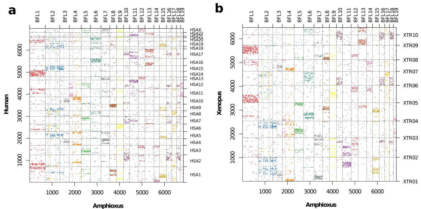
Extended Data Fig. 2 | Dot-plots showing conserved synteny between amphioxus and human and frog. Dots represent mutual best hits between amphioxus and frog ( Xenopus tropicalis , XTR) and human ( Homo sapiens , HSA). Only mutual-best-hits involving the 6,843 genes of Fig. 1 are considered. (These gene families are anchored by mutual best hits between the four jawed vertebrate representatives and amphioxus.) Genes are colored based on their CLG membership as in main Fig. 1. Horizontal and vertical solid lines represent chromosome boundaries; vertical dashed lines represent inferred syntenic breakpoints in amphioxus as in Fig. 1 (Methods).
