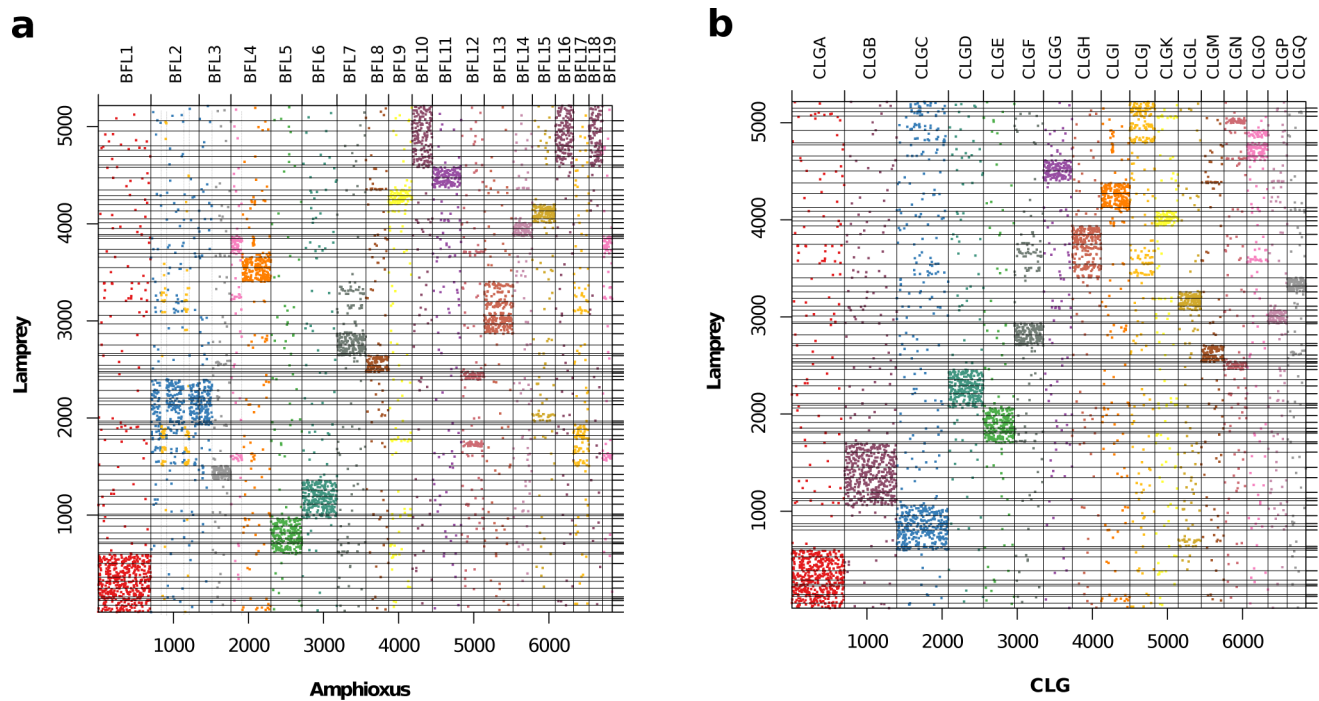
Extended Data Fig. 3 | Dot-plots showing conserved syntenies between lamprey and amphioxus. Dots represent mutual best hits between the (germline) genome of the sea lamprey ( Petromyzon marinus ) and amphioxus. Genes are colored based on their CLG assignment, and lamprey chromosomes are sorted according to their CLG content. Panel a shows these distribution of orthologous genes vs. amphioxus chromosomes, revealing the same discontinuities (vertical dashed lines) in amphioxus-lamprey synteny as found for amphioxus-bony vertebrate comparisons shown in Fig. 1 and Extended Data Fig. 2. Panel b shows these same orthologous gene pairs versus CLGs.
