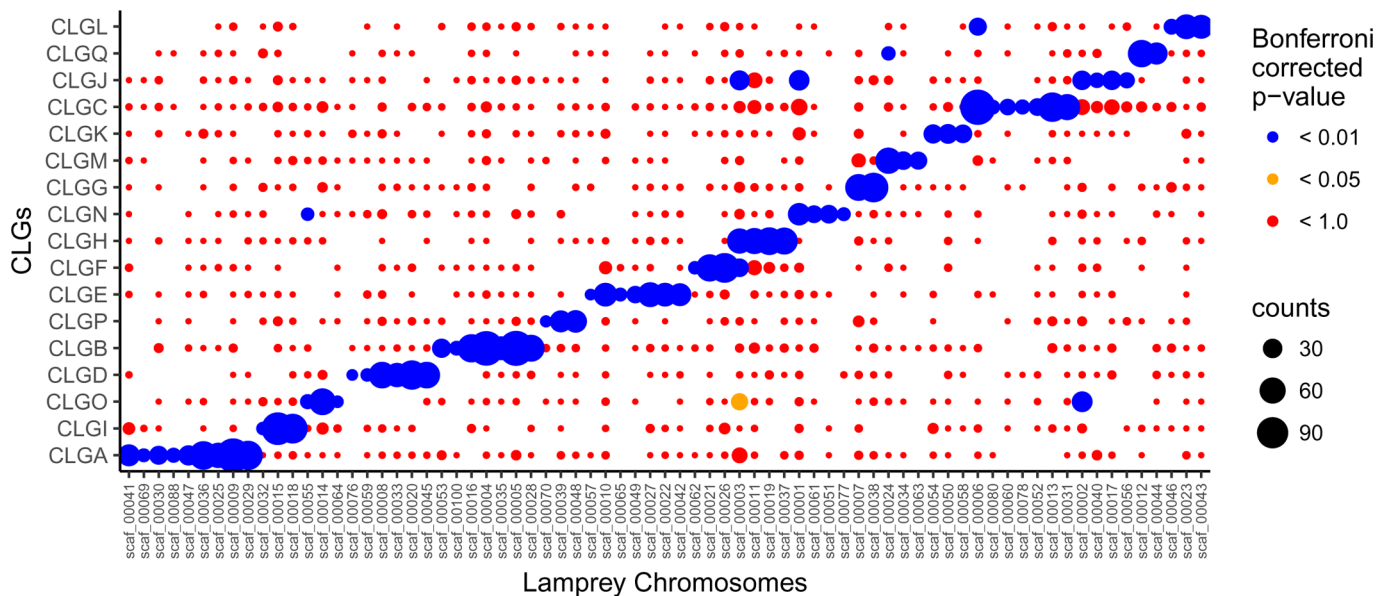
Extended Data Fig. 8 | Oxford grid between sea lamprey germline chromosomes and chordate linkage groups (CLGs). Circles show the number of orthologous genes between germline chromosomes of sea lamprey ( Petromyzon marinus , PMA, denoted scaff_XXXXX following Smith et al.) and the seventeen CLGs described in the main text. As in Extended Data Fig. 6 the area of each circle is proportional to the number of orthologous genes for each chromosome-CLG pair, and the color indicates the significance of the association relative to a null model in which the position of the orthologous genes are randomly shuffled. Sea lamprey chromosomes and CLGs are both sorted to exhibit the striking correspondence between them. Each of the 17 CLGs is represented by at least one lamprey chromosome, and typically 6-8 lamprey chromosomes are associated with each CLG. Compare Fig. 4b of Smith and Keinath 2015, which compares lamprey chromosomes to 'putative ancestral linkage groups' derived by Putnam 2008 through clustering of amphioxus scaffolds. These putative ancestral linkage groups are in 1:1 correspondence with the CLGs shown here to be represented as large chromosomal segments of amphioxus.
