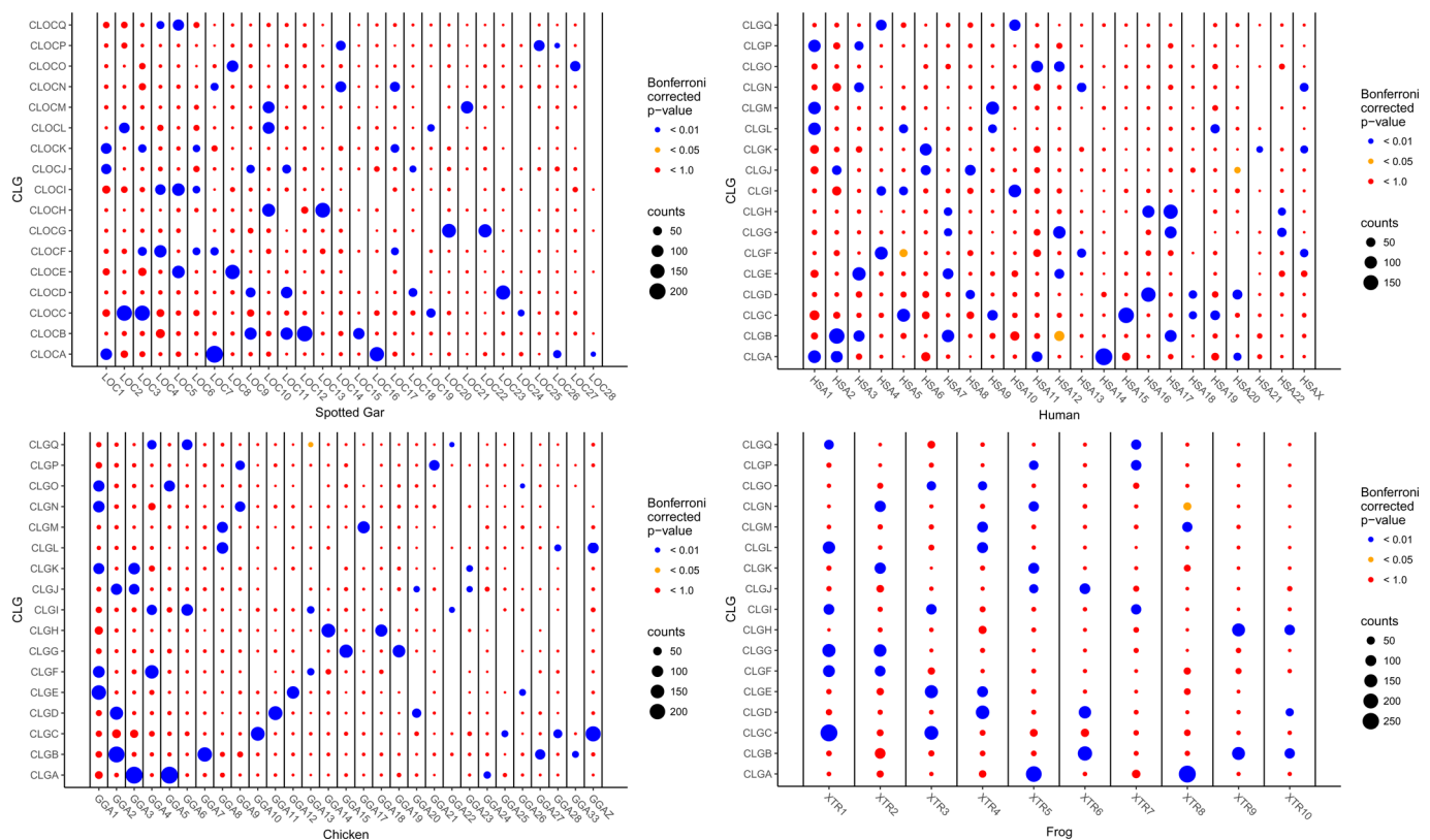
Extended Data Fig. 6 | Oxford grid between bony vertebrate chromosomes and chordate linkage groups (CLGs). Circles represent the number of orthologous genes between human ( Homo sapiens , HSA), chicken ( Gallus gallus , GGA), frog ( Xenopus tropicalis , XTR), and spotted gar ( Lepisosteus oculatus , LOC) and the seventeen chordate linkage groups (CLGs) described in the text. Orthology is operationally defined by mutual best hits, restricted to 6,843 gene families anchored by mutual best hits of the four jawed vertebrates to amphioxus. The area of each circle is proportional to the number of orthologous genes for each chromosome-CLG pair, and the color indicates the significance of the association relative to a null model in which the position of the orthologous genes are randomly shuffled (Methods).
