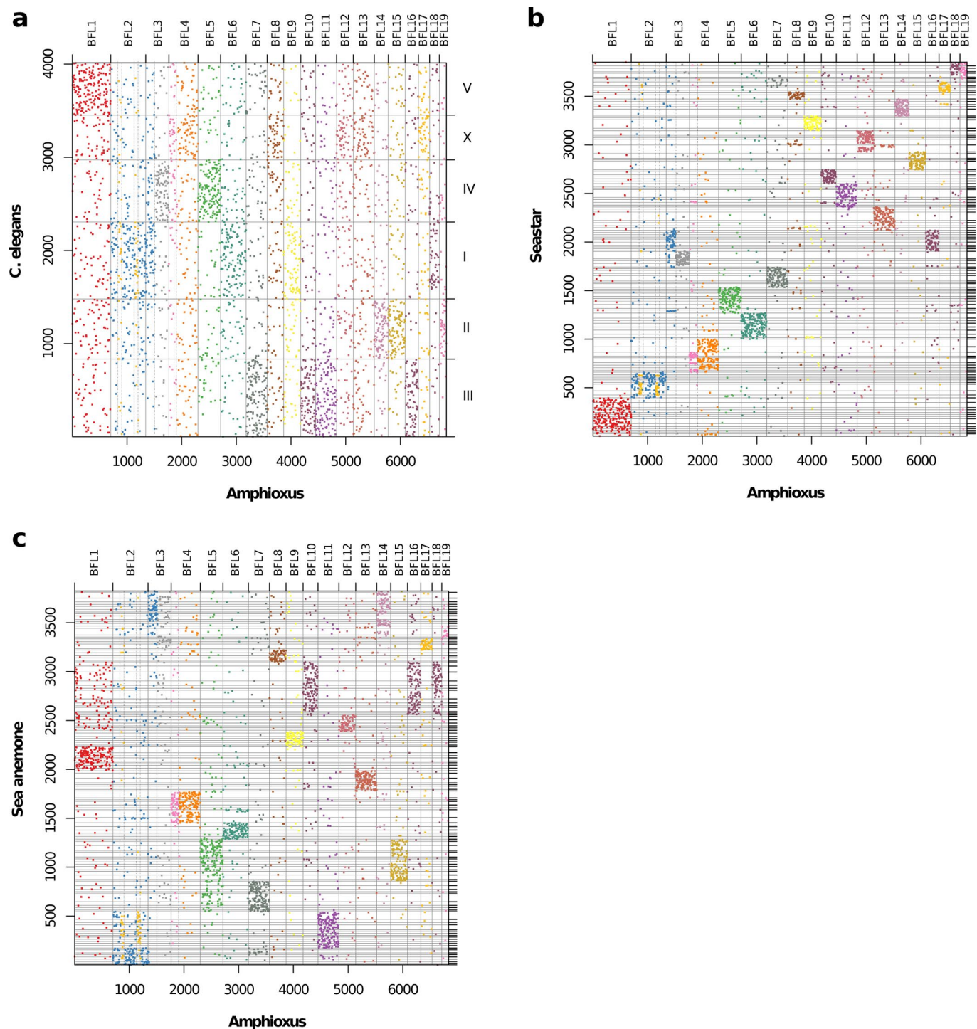
Extended Data Fig. 4 | Dot-plots showing conserved synteny between amphioxus and selected invertebrates. Dots represent mutual best hits between amphioxus and the genomes of the Crown Of Thorns sea star Acanthaster planci , the soil nematode Caenorhabditis elegans , and the starlet sea anemone Nematostella vectensis . The N. vectensis and A. planci genomes are not yet assembled into chromosomes, and only scaffolds containing 20 or more genes (counting only mutual-best-hit vs. amphioxus) are shown. Scaffolds are sorted based on clustering using similarity of their CLG content. Vertical dashed lines are as shown in and Fig. 1, with the same CLG-based coloring, showing that the partitioning of amphioxus found using jawed vertebrates is also consistent with diverse invertebrates, and that sea star and sea anemone scaffolds can be grouped according to conserved synteny with amphioxus. C. elegans chromosomes arose by fusion, translocation, and mixing of the ancestral bilaterian units that are still retained in amphioxus.
