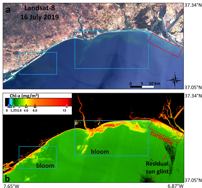
Figure 8. (a) Landsat-8 RGB (bands 4-3-2) composite in the study region on 16 July 2019 showing the L. polyedra algal bloom located in the waters off the Guadiana estuary mouth (contains modified Copernicus Sentinel data 2019 processed by Sentinel Hub); (b) chl-a concentration ( \text{mg}/\text{m}^3 ) after atmospheric correction with ACOLITE for the same scene. Some residual sun glint after atmospheric correction is visible in the lower right panel of the chl-a map (black pixels). Blue rectangles indicate high concentrations of chl-a due to the algal bloom, whereas the red rectangle indicates a high chl-a concentration due to high turbidity in the Tinto-Odiel estuary (Ria de Huelva and Punta Umbria, Fig. 1b). Maps are generated by SNAP 7.0.0 ( https://step.esa.int/main/download/snap-download/ ). L8 image was downloaded from Earth Explorer ( https://earthexplorer.usgs.gov/ ) and processed with ACOLITE 20190326.0 ( https://odnature.naturalsciences.be/remsem/software-and-data/acolite ).
