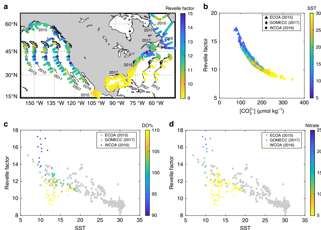
Fig. 4 Revelle factor in the North Atlantic margins. a Spatial distribution of the Revelle factor, b correlation of the Revelle factor to [\text{CO}_3^{2-}] , and c , d correlation of the Revelle factor to SST color coded by DO% and [\text{NO}_3^-] . Spatial distribution of [\text{CO}_3^{2-}] is presented in Supplementary Fig. 4. In c , d , only the CCS data are color coded.
