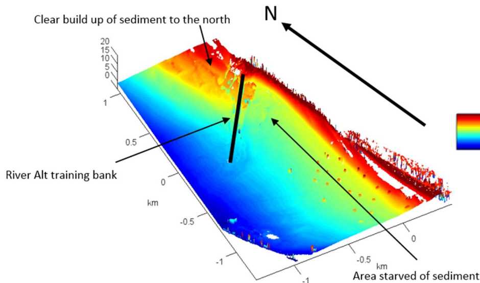
Figure 12: Intertidal elevation analysis December 2016 at Crosby, UK (Image provided by Marlan Maritime Technologies Ltd)
