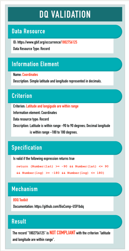
Figure 6. Example of a data quality validation.
