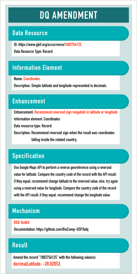
Figure 7. Example of a data quality amendment.
