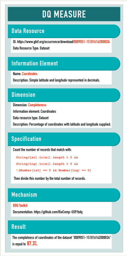
Figure 5. Example of a data quality measure.
