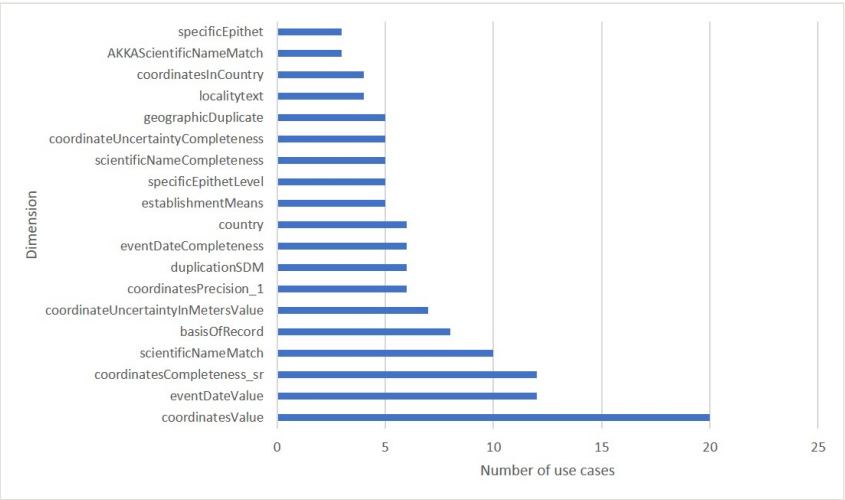
Figure 13. Number of use cases associated with each Dimension (for a full list of dimensions, see Suppl. material 2). Dimensions that had fewer than three associated use cases are not shown.
