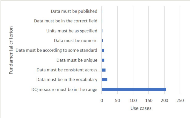
Figure 10. Number of use cases associated with each fundamental criterion (see Suppl. material 2). As each use case can be associated with multiple criteria, use cases may be double counted when criteria are combined to form fundamental criterion.
