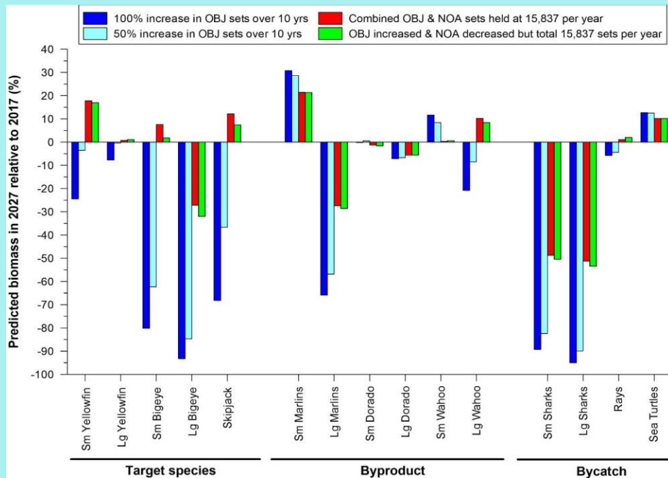
Figure 30 Ecosim predicted relative changes in the biomass of key functional groups representing primary target species, byproduct, and bycatch of the purse-seine fishery in the eastern tropical Pacific Ocean in 2027 relative to 2017 under four hypothetical management scenarios
