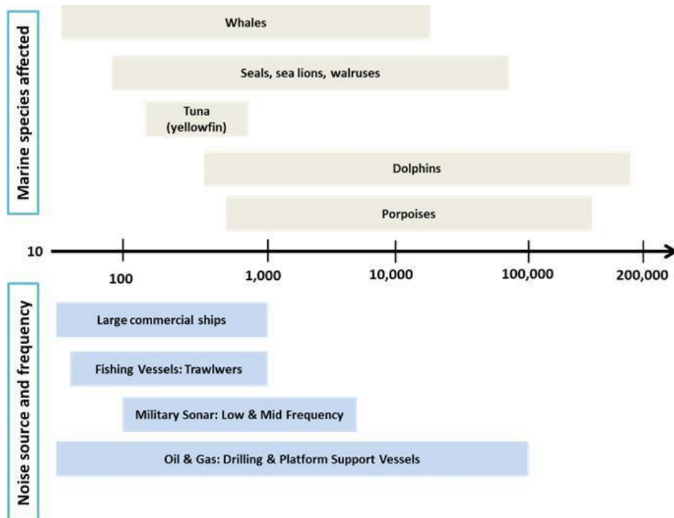
Figure 37 Audiogram for selected species and ship types
