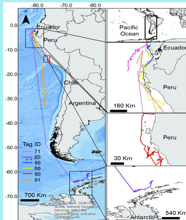
Figure 14 Migration of humpback whales from Ecuador to Antarctic waters
