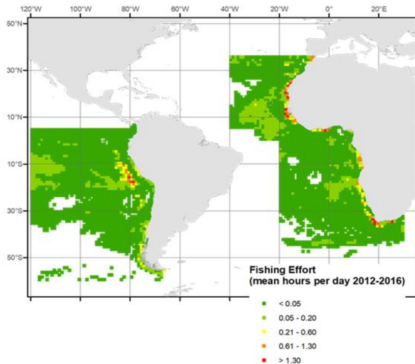
Figure 22 Fishing effort in the Southeast Atlantic and Southeast Pacific (2012 – 2016) (mean hours per day) Source: Global Fishing Watch, 2019
