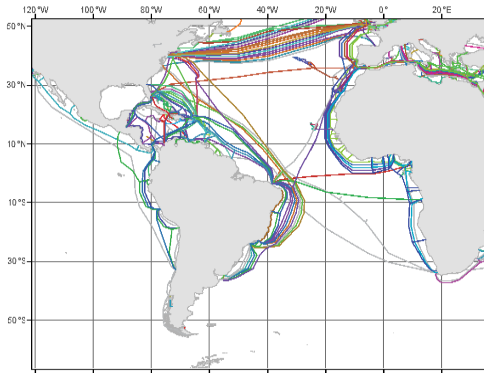
Figure 31 Submarine cables in the Southeast Atlantic and Southeast Pacific
