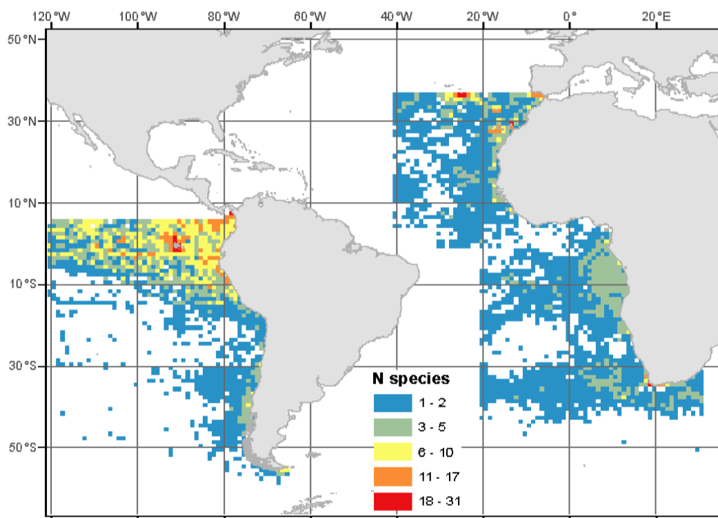
Figure 11 Megafauna species richness Source: OBIS SEAMAP, 2019 26
