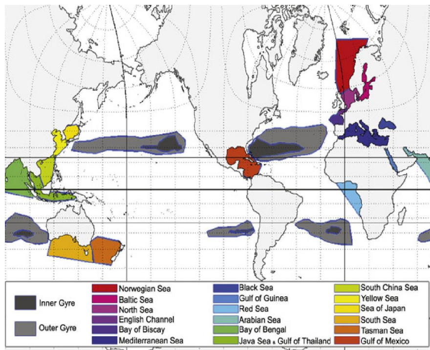
Figure 32 The accumulation of floating material after 30 years of simulated input and circulation. Map showing the boundaries of the various accumulations zones
