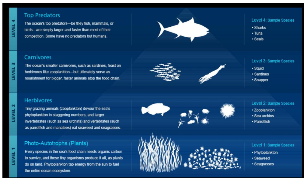
Figure 8 Marine food chain levels
