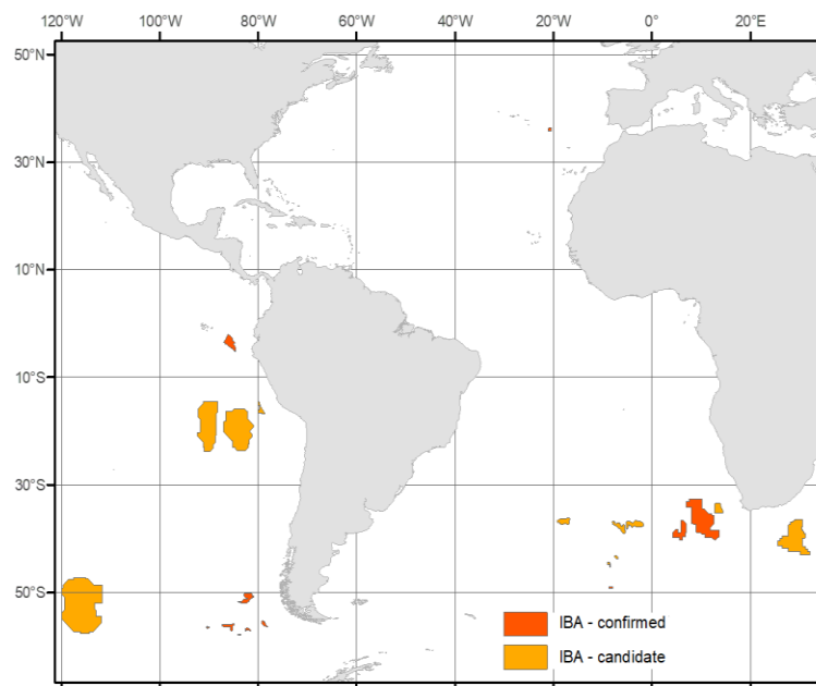
Figure 18 Location of marine confirmed and candidate IBAs in the Southeast Atlantic and Southeast Pacific
