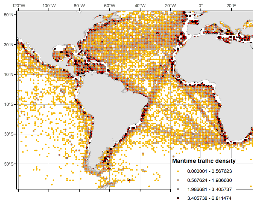
Figure 35 Maritime traffic density in the Southeast Atlantic and the Southeast Pacific
