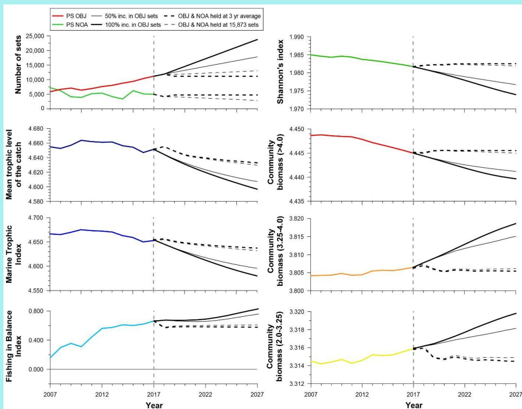
Figure 29 Estimated changes in annual values for seven ecological indicators after the simulation of four hypothetical scenarios changing the effort of the purse-seine fishery on floating objects (or OBJ) over a 10-year period initiated in 2017 and concluding in 2027
