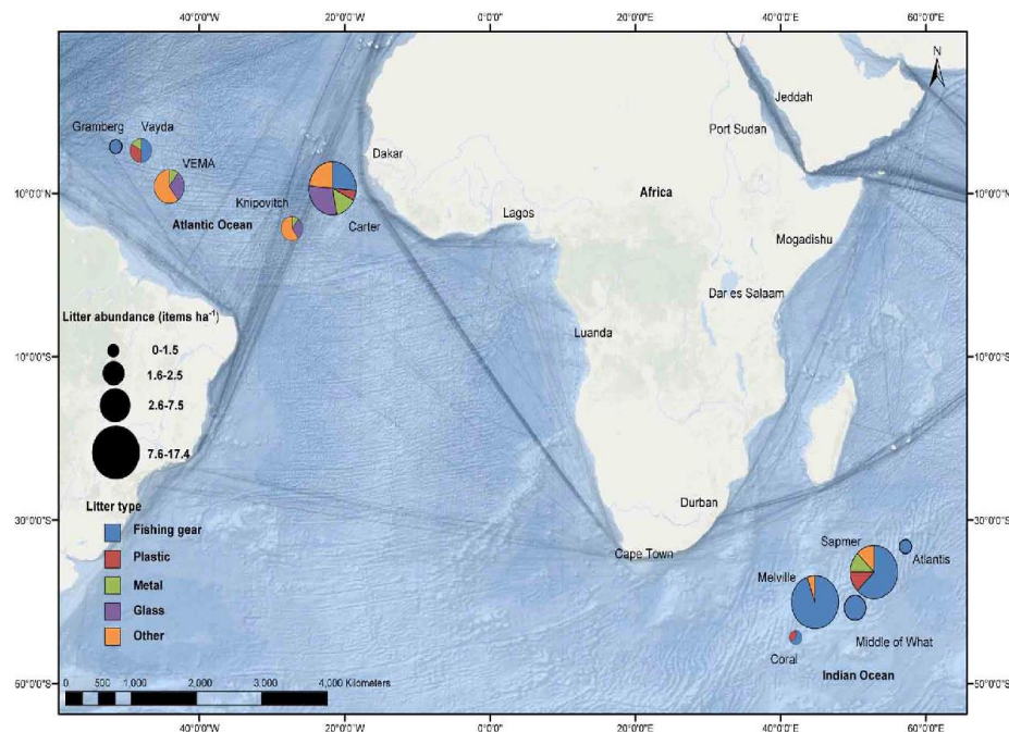
Figure 33 Survey locations benthic litter densities (itemsha -1 ) and composition for individual submarine features observed by remotely operated vehicle video systems. Commercial shipping activity is overlaid with the darkest lines representing areas with greatest shipping activity
