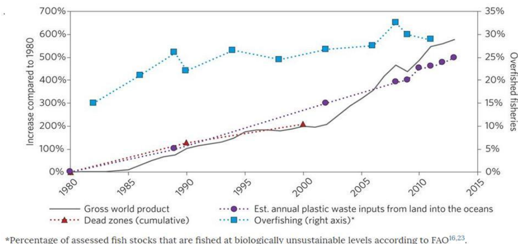
Figure 1 Trends in gross world product, overfishing and ocean pollution
