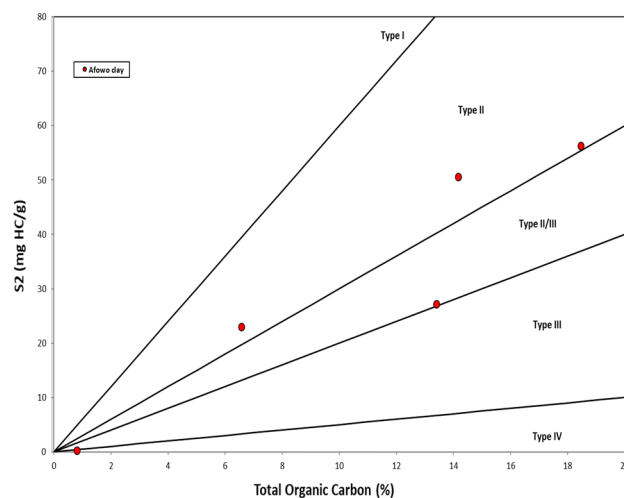
Figure 10. Cross plot of S2 against TOC showing kerogen type. The outlier with almost nil S2 and TOC represented the claystone at a depth of 8.7 m (Adapted from Mohammed et al. 11 ). The organic matter types indicated sedimentation in both marine and terrestrial environments.
